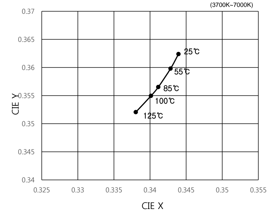
Fig 8. Chromaticity Coordinate vs. Junction Temperature, I_F=120\text{mA}
