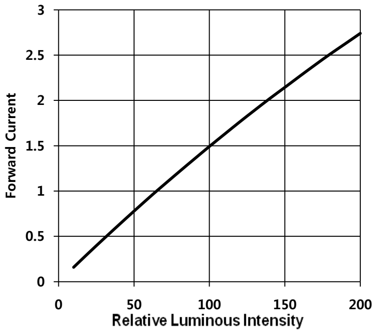
Fig 4. Forward Current vs. Relative Luminous Intensity, T_j = 25^\circ\text{C}
