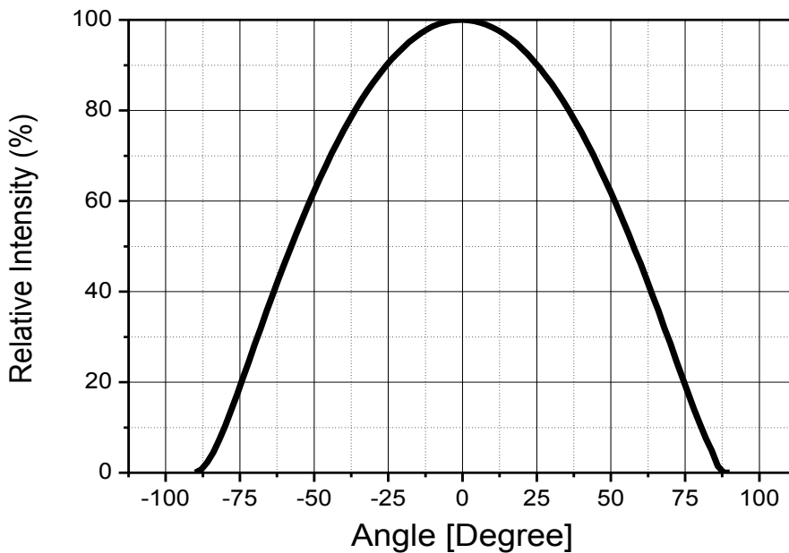
Fig 2. Radiant Pattern, T_j = 25^\circ\text{C} , I_F = 65\text{mA}
