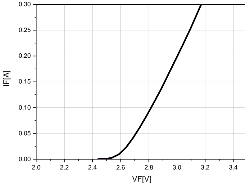
Fig 3. Forward Voltage vs. Forward Current, T_j = 25^\circ\text{C}
