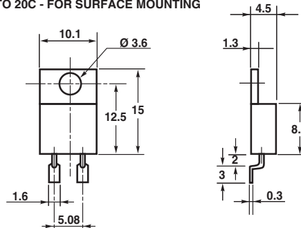
RTO 20C - FOR SURFACE MOUNTING
