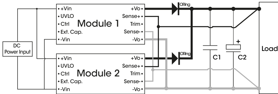
Figure 11. Multiple Modules Connected in Parallel
