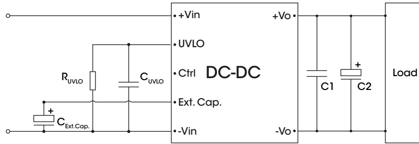
Figure 10. Recommended circuit for external hold-up capacitor
