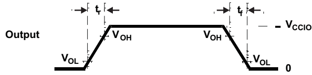
Figure 4-3. CMOS-Level Outputs
