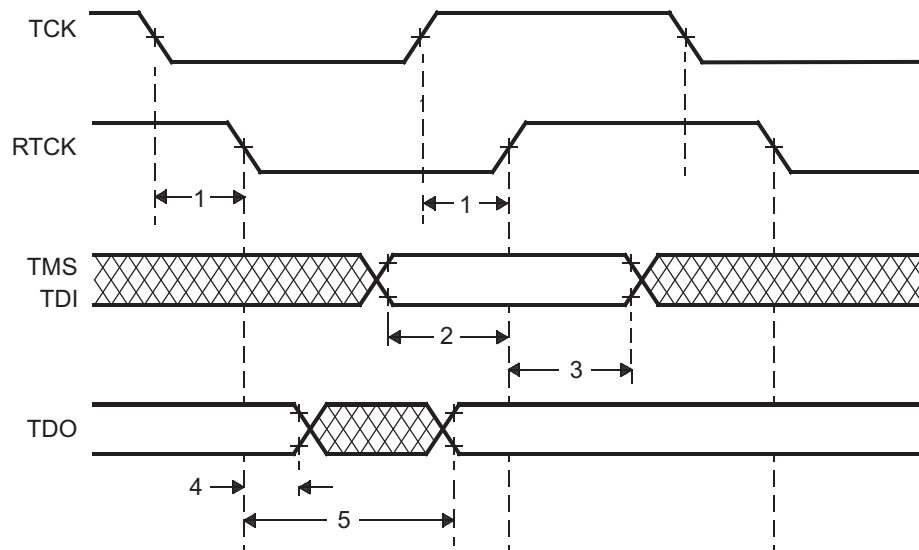
Figure 5-14. JTAG Timing
