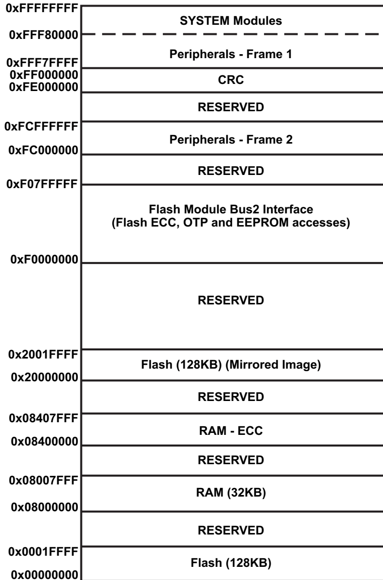
Figure 5-9. RM41232 Memory Map
