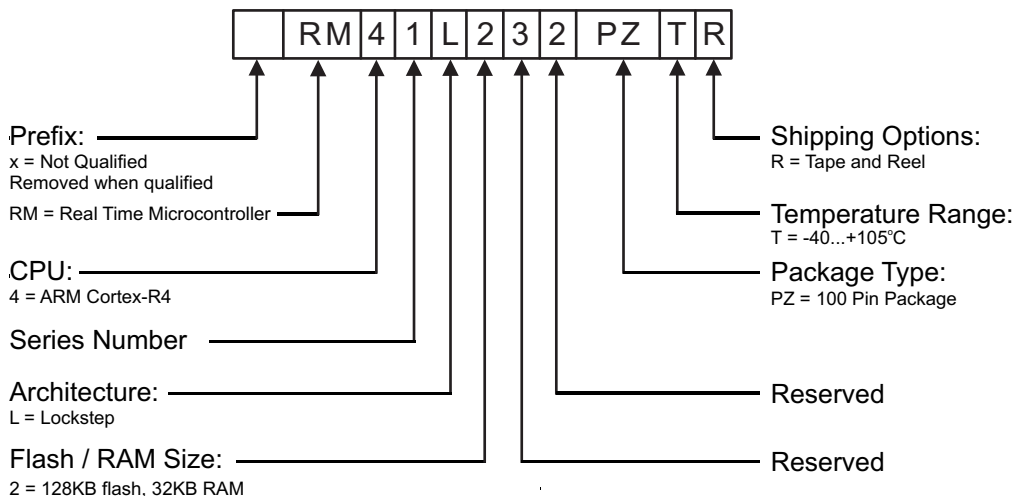
Figure 7-1. Device Numbering Conventions
