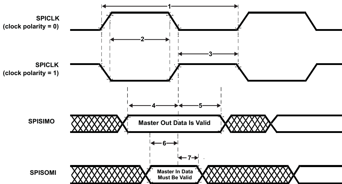
Figure 6-6. SPI Master Mode External Timing (CLOCK PHASE = 0)
