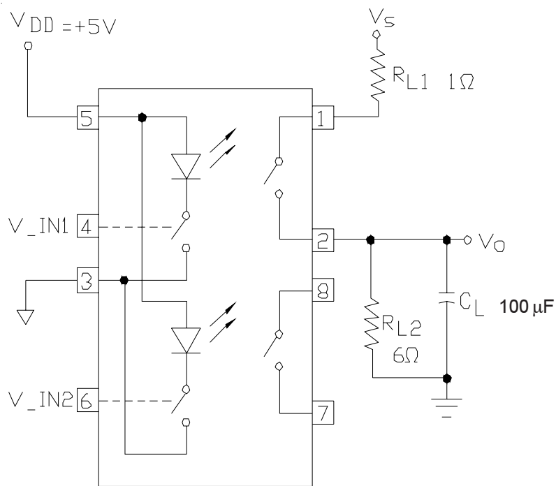
Fig 3: Switching Test Circuit (Only one channel shown)
