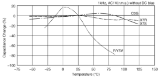
Capacitance - temperature characteristics
