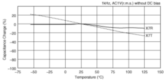
Capacitance - temperature characteristics
