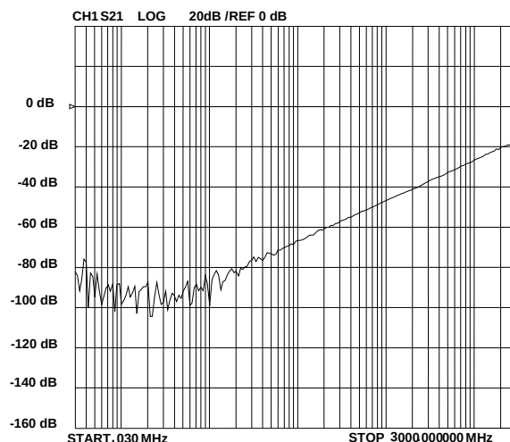
Analog Crosstalk DM, DP, ID Pins (Pins 2, 3, 4)
