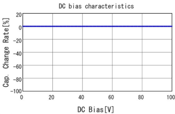
■ RCE5C2A220J0A2H03B C-DC bias capchange, 25.0degC, AC1
