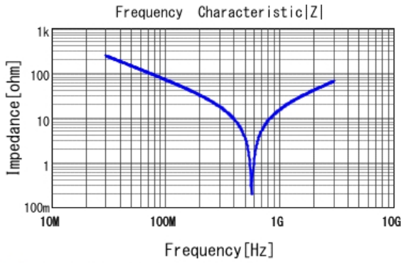
■ RCE5C2A220J0A2H03B |Z| DCOV, 25degC
