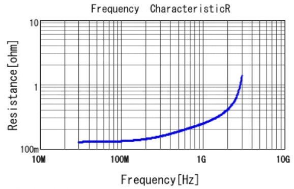
■ RCE5C2A220J0A2H03B R DCOV, 25degC
