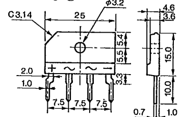
Outline Drawing 71
