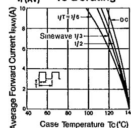
I F(AV) - T c Derating
