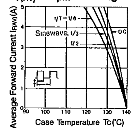
I F(AV) - T pin Derating
