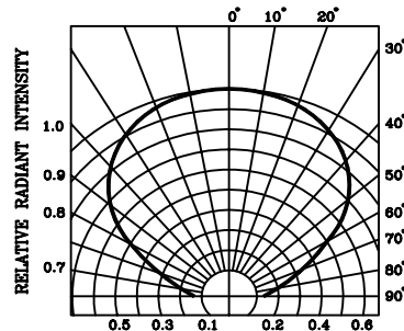
Fig.6 RADIATION DIAGRAM RADIATION DIAGRAM
