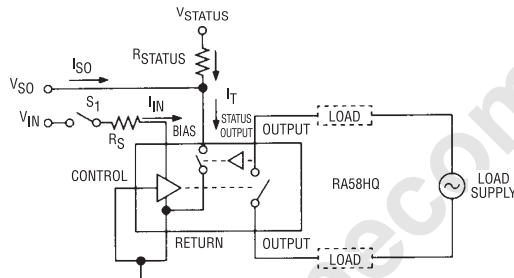
(C) 2 TERMINAL INPUT (DIRECT DRIVE) WITH STATUS
