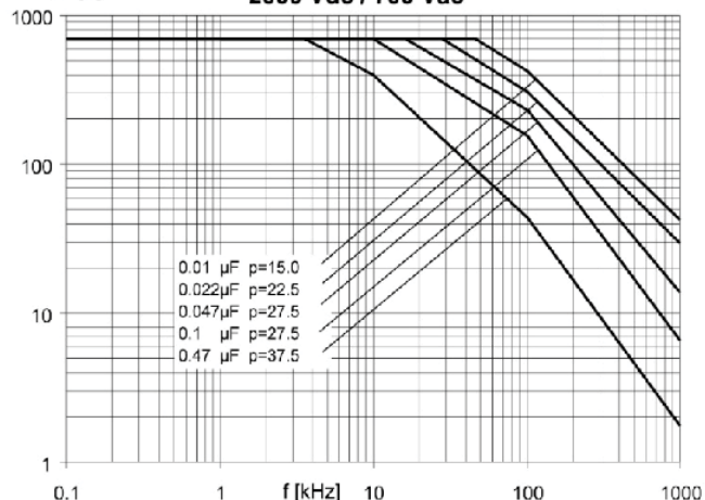
2000 Vdc / 700 Vac
