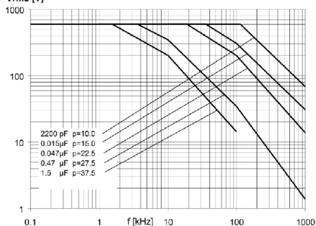
1000 Vdc / 600 Vac
