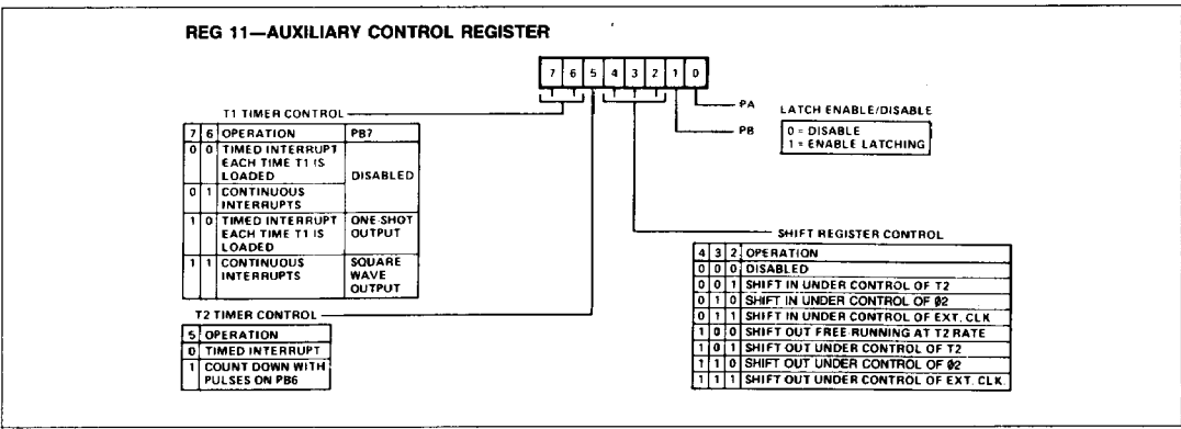
Figure 14. Auxiliary Control Register (ACR)
