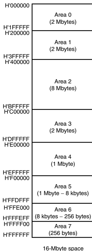
Figure 6.7 Address Space Area Division
