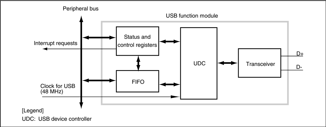
Figure 15.1 Block Diagram of USB
