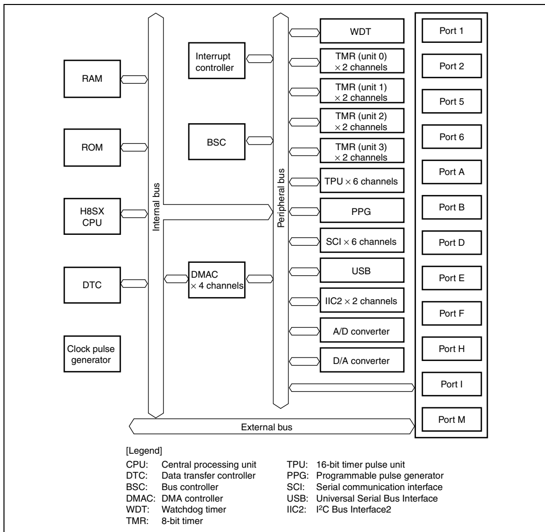
Figure 1.1 Block Diagram
