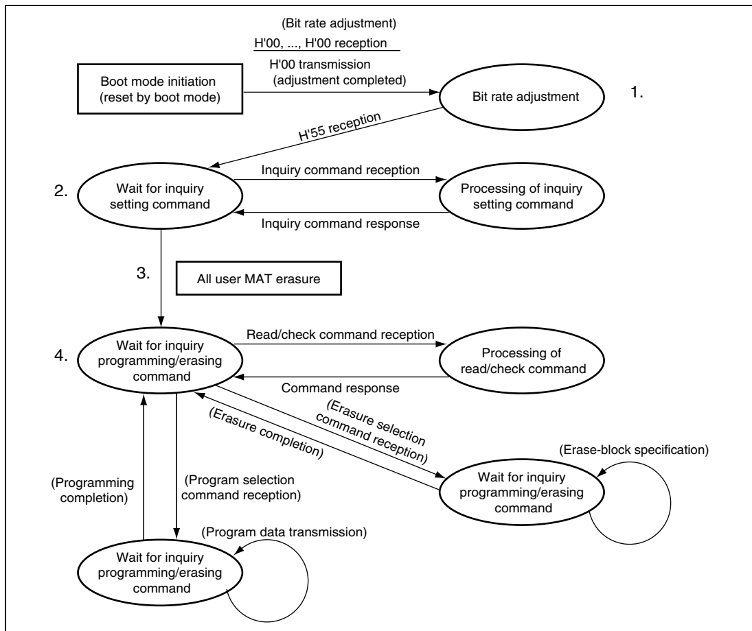
Figure 20.8 SCI Boot Mode State Transition Diagram
