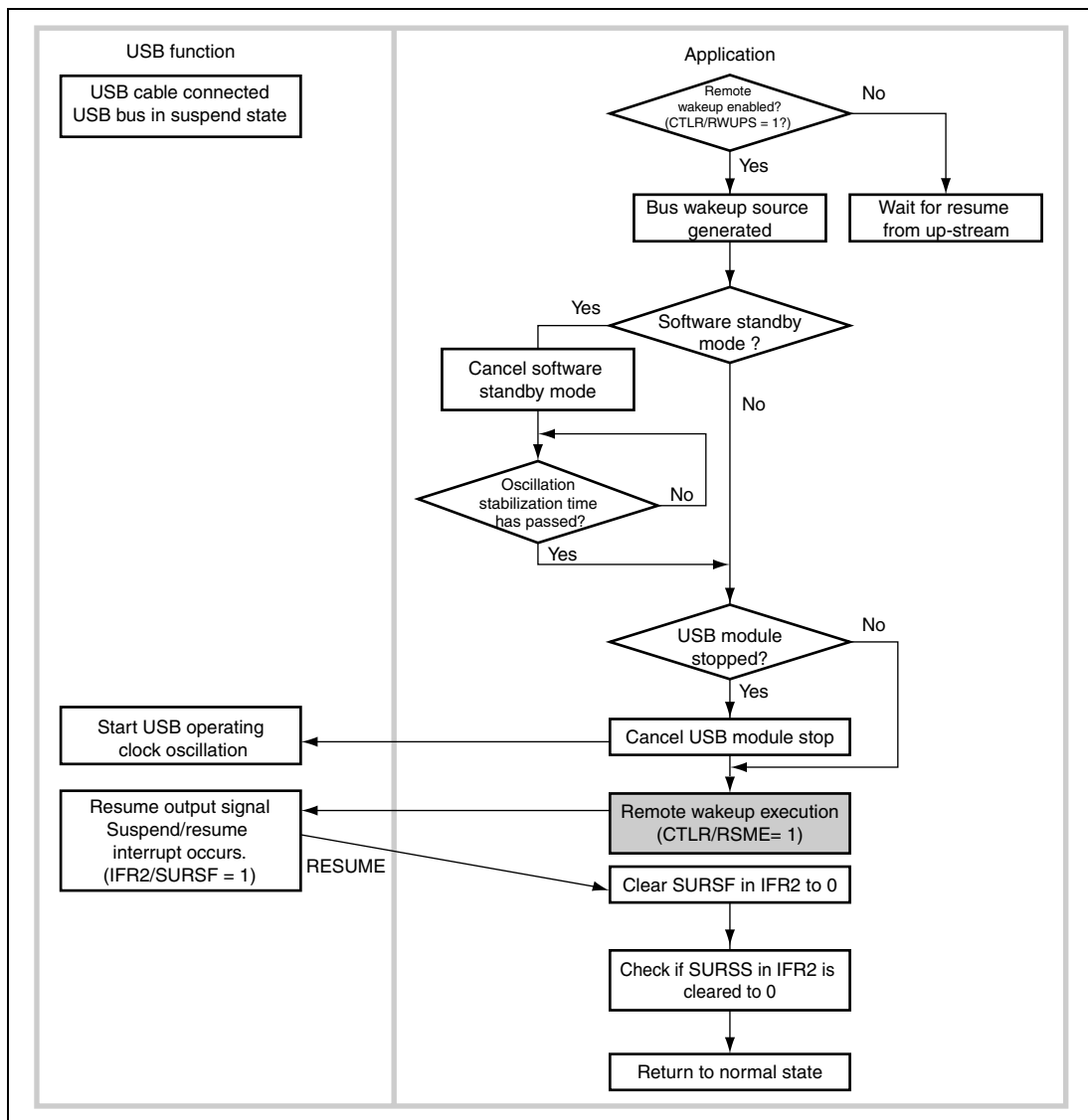
Figure 15.8 Remote-Wakeup
