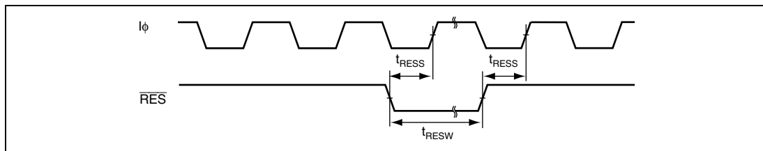
Figure 24.6 Reset Input Timing
