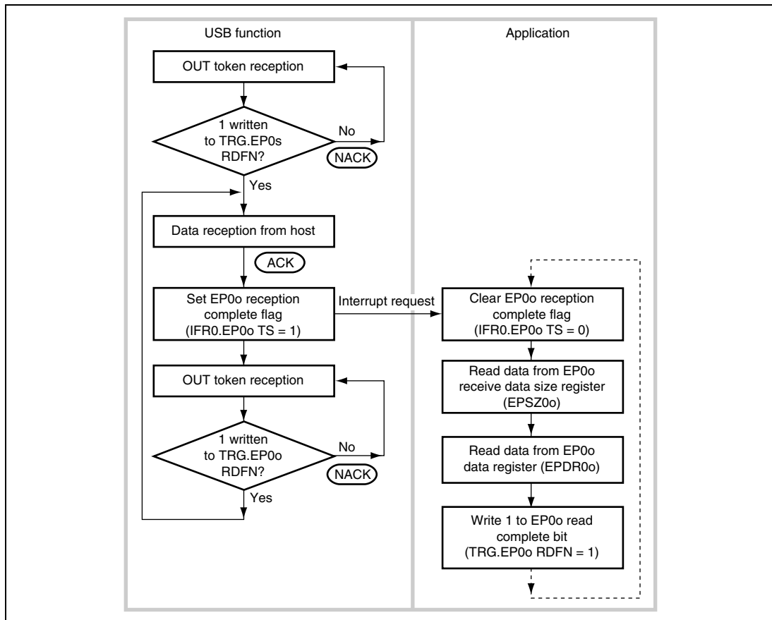
Figure 15.12 Data Stage (Control-Out) Operation
