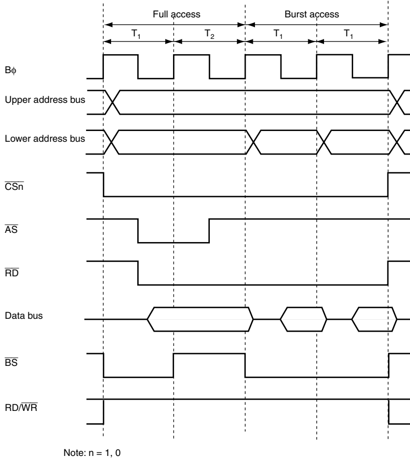
Figure 6.29 Example of Burst ROM Access Timing ( ASTn = 0 , One Burst Cycle)
