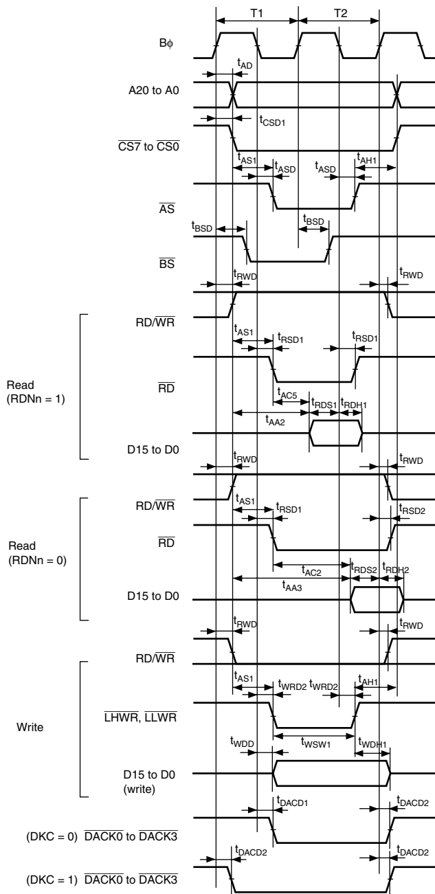
Figure 24.8 Basic Bus Timing: Two-State Access
