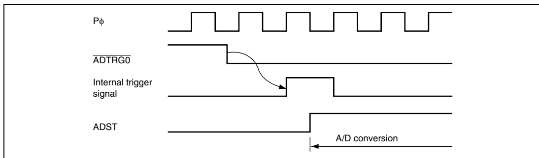
Figure 17.5 External Trigger Input Timing
