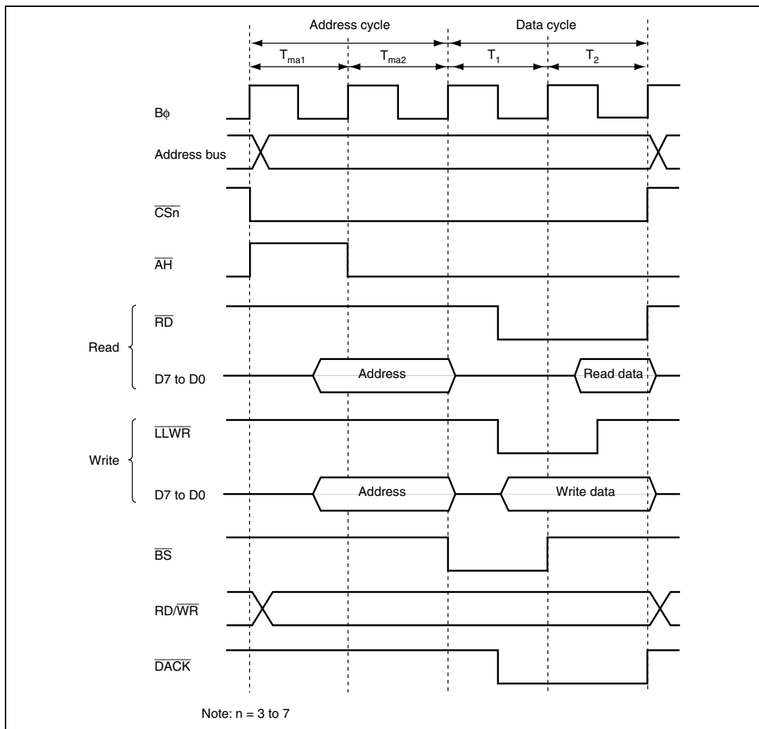
Figure 6.30 8-Bit Access Space Access Timing (ABWHn = 1, ABWLn = 1)
