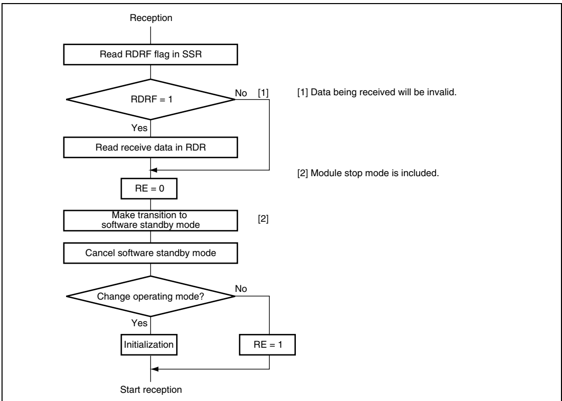
Figure 14.42 Sample Flowchart for Mode Transition during Reception
