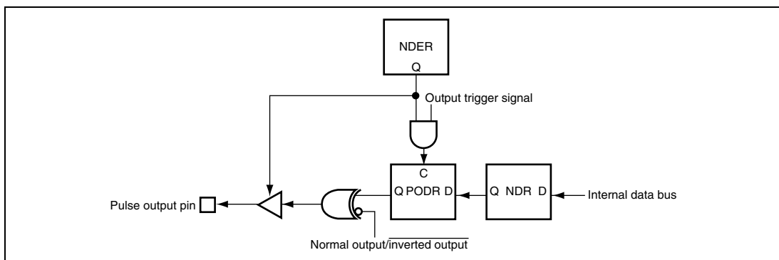
Figure 11.2 Schematic Diagram of PPG
