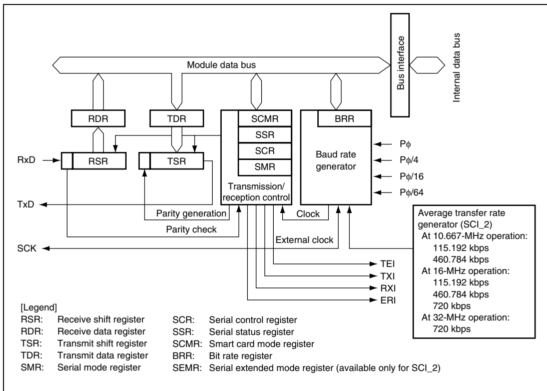
Figure 14.1 Block Diagram of SCI_0, 1, 2, and 4
