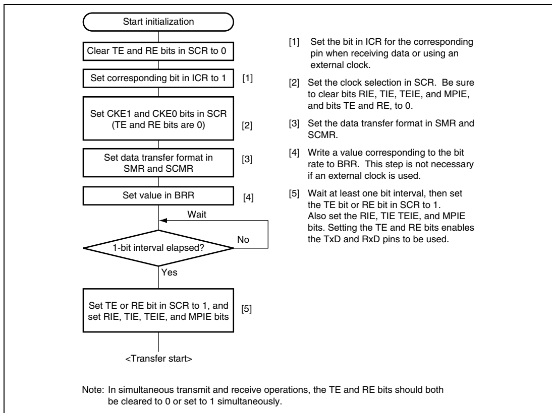
Figure 14.18 Sample SCI Initialization Flowchart
