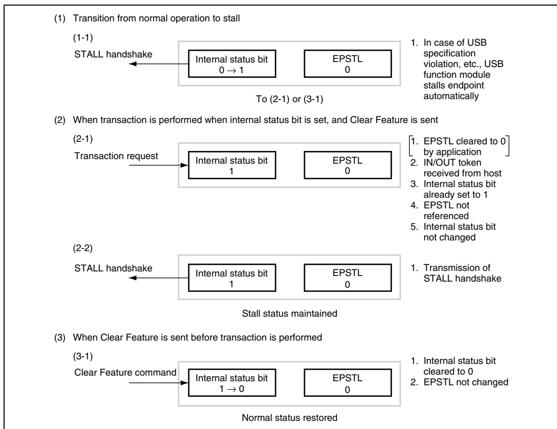
Figure 15.19 Automatic Stall by USB Function Module
