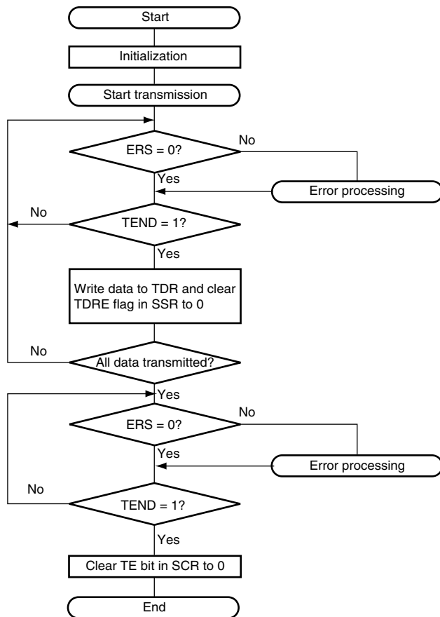
Figure 14.31 Sample Transmission Flowchart
