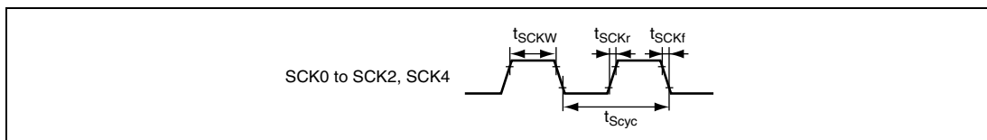
Figure 24.33 SCK Clock Input Timing
