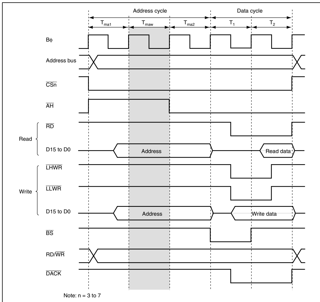
Figure 6.32 Access Timing of 3 Address Cycles (ADDEX = 1)
