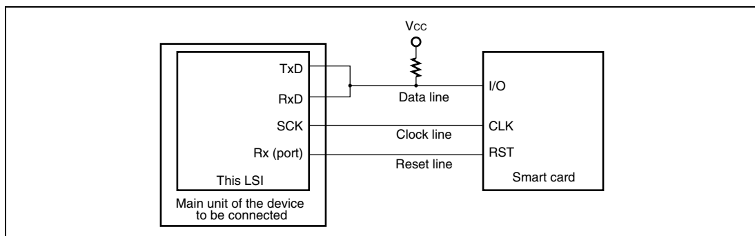
Figure 14.24 Pin Connection for Smart Card Interface
