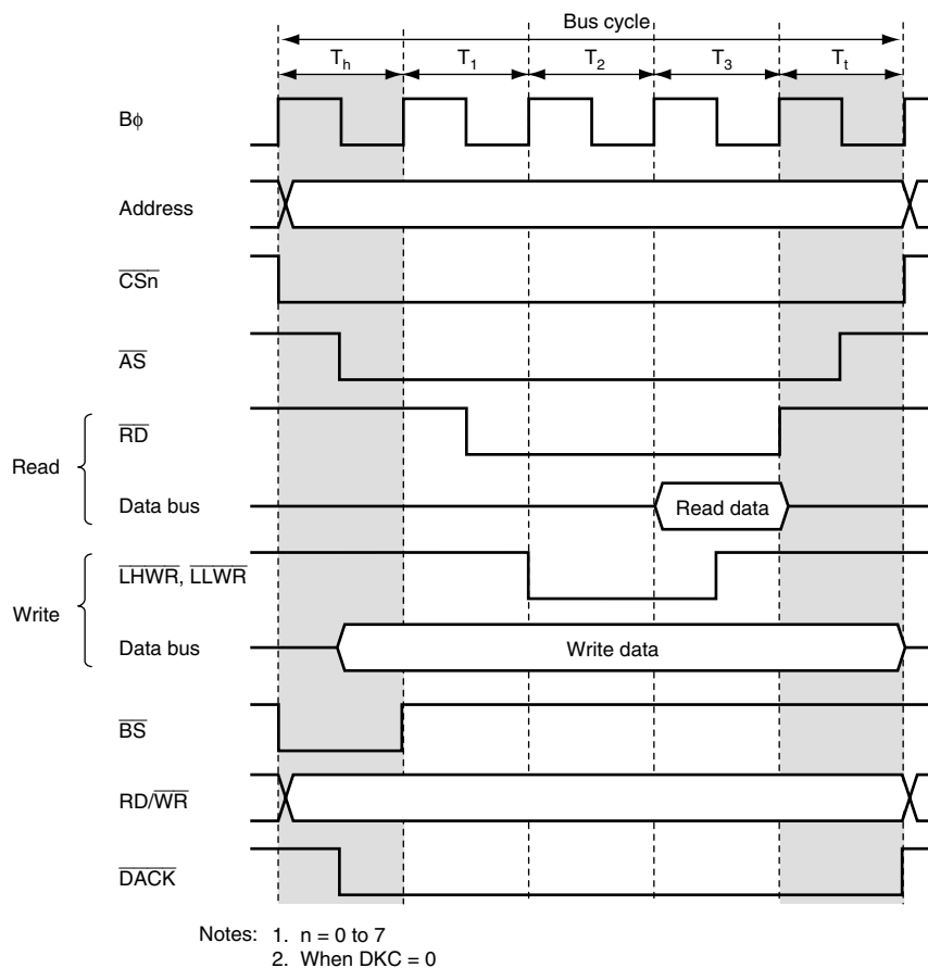
Figure 6.22 Example of Timing when Chip Select Assertion Period is Extended
