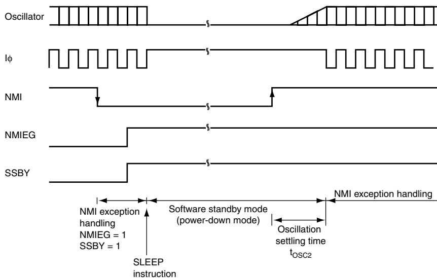
Figure 24.3 Oscillation Settling Timing after Software Standby Mode
