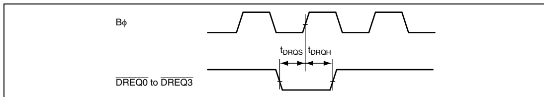
Figure 24.21 DMAC ( \overline{DREQ} ) Input Timing
