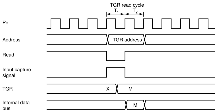
Figure 10.50 Conflict between TGR Read and Input Capture
