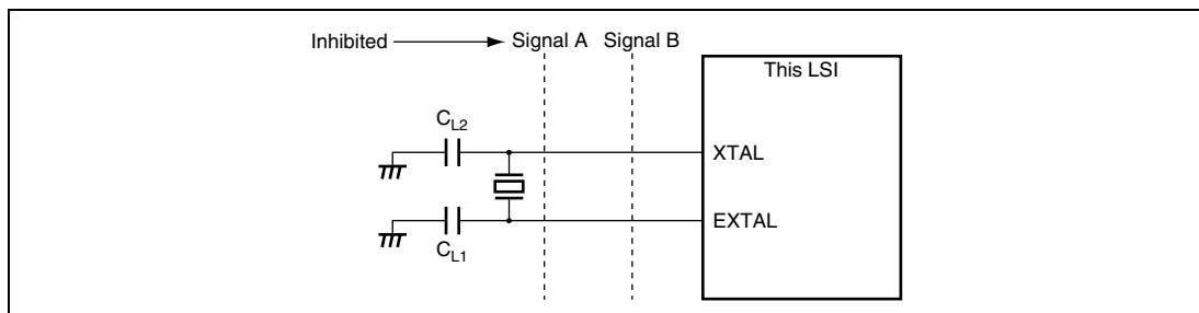
Figure 21.7 Note on Board Design for Oscillation Circuit
