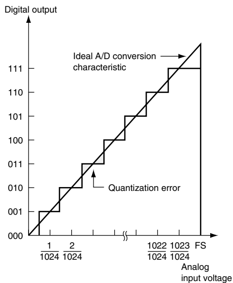
Figure 17.6 A/D Conversion Accuracy Definitions
