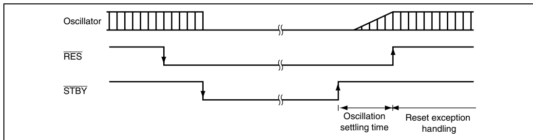
Figure 22.3 Hardware Standby Mode Timing
