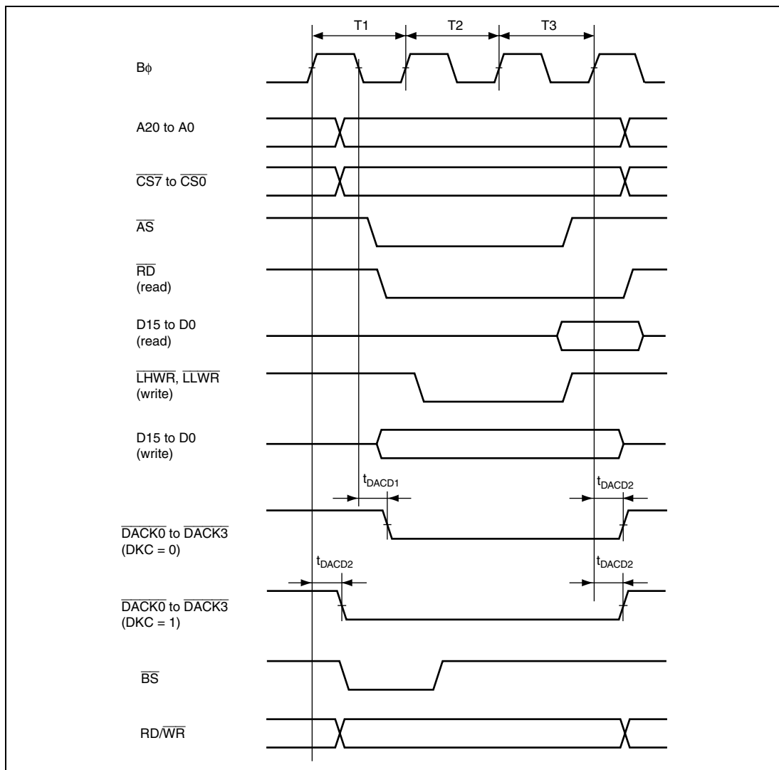
Figure 24.24 DMAC Single-Address Transfer Timing: Three-State Access
