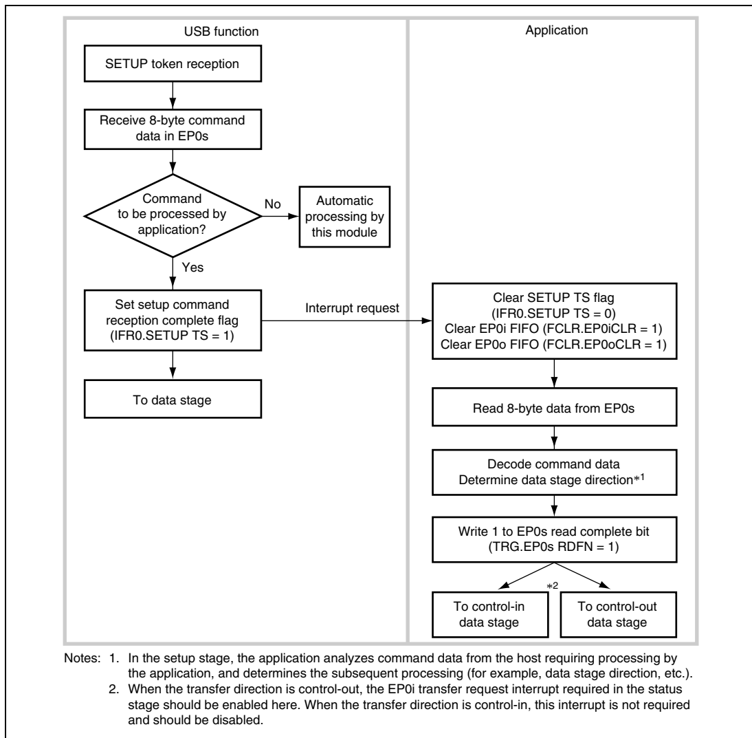
Figure 15.10 Setup Stage Operation
