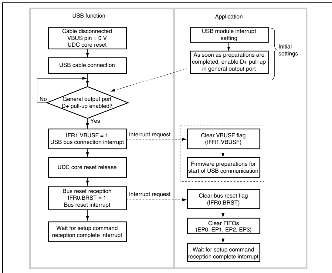
Figure 15.2 Cable Connection Operation
