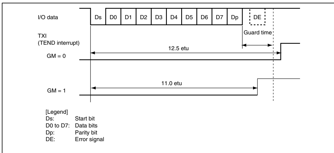
Figure 14.30 TEND Flag Set Timing during Transmission
