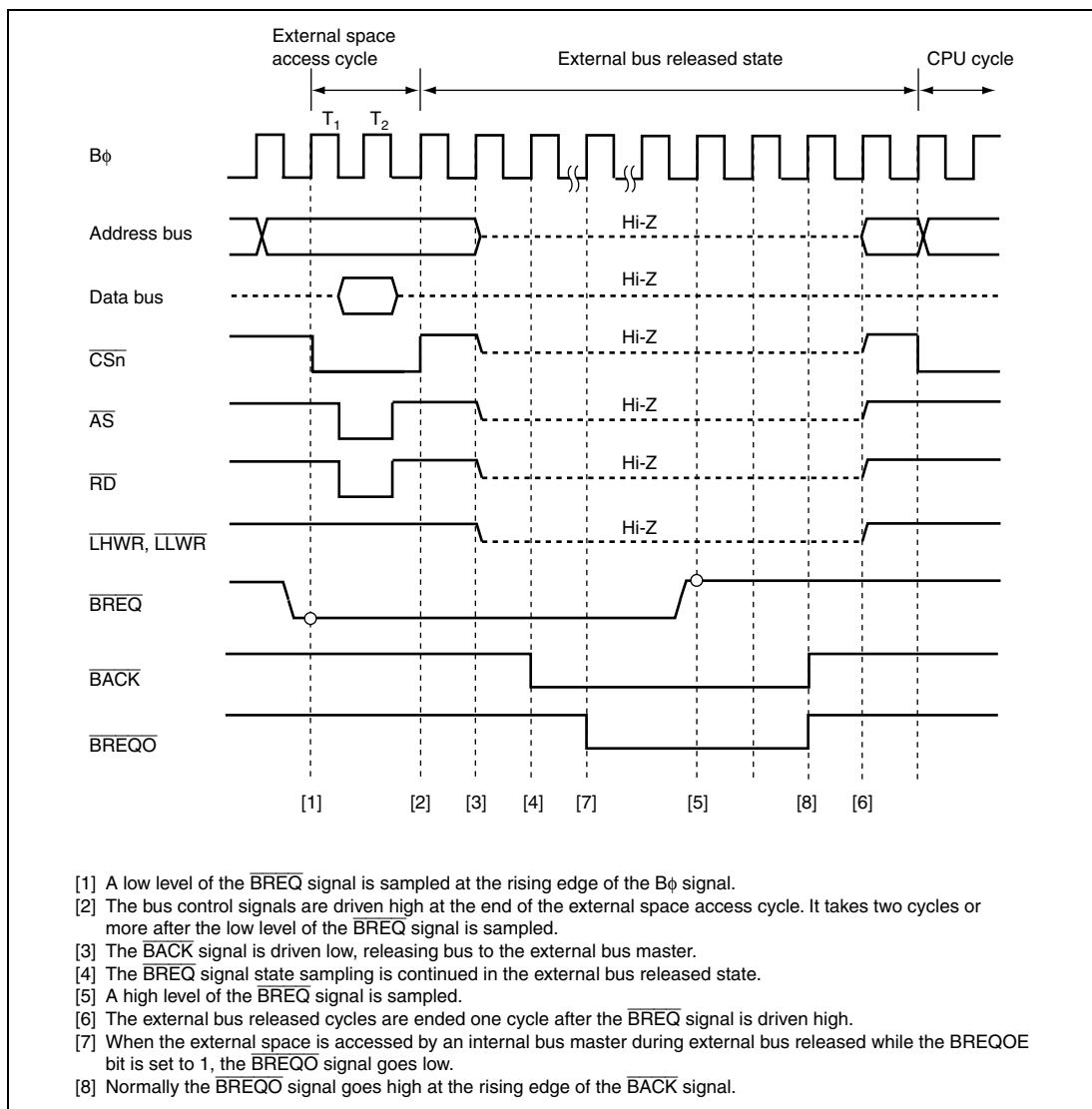
Figure 6.43 Bus Released State Transition Timing
