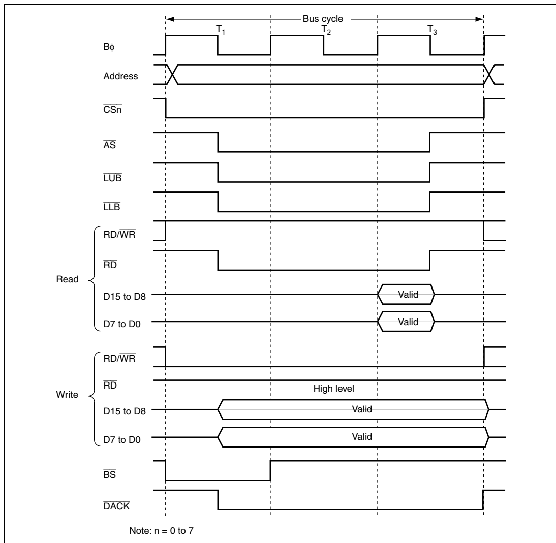
Figure 6.25 16-Bit 3-State Access Space Bus Timing
