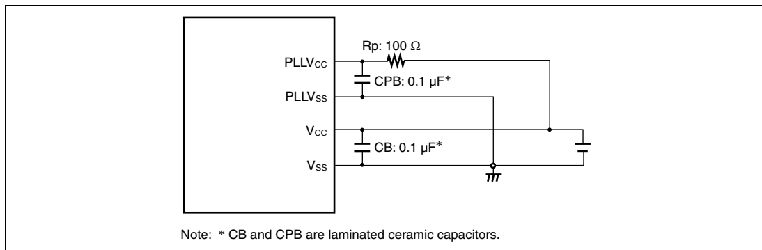
Figure 21.8 Recommended External Circuitry for PLL Circuit
