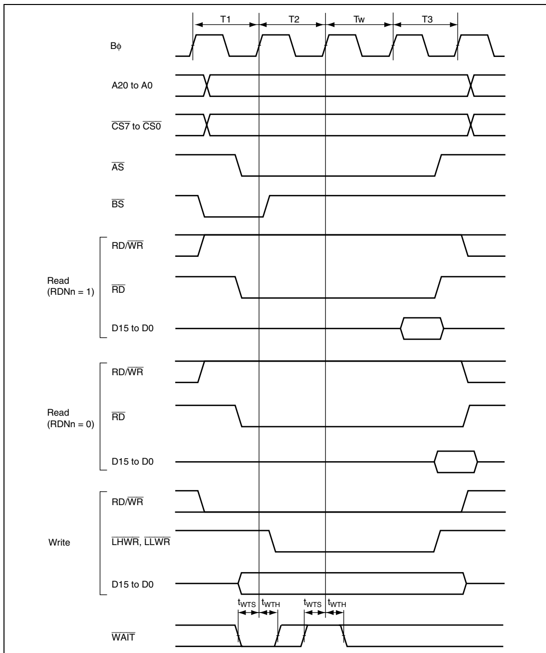
Figure 24.10 Basic Bus Timing: Three-State Access, One Wait
