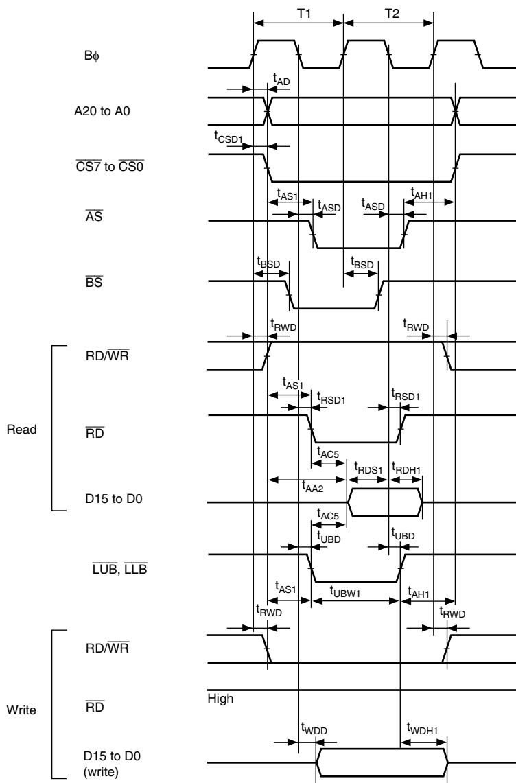
Figure 24.13 Byte Control SRAM: Two-State Read/Write Access
