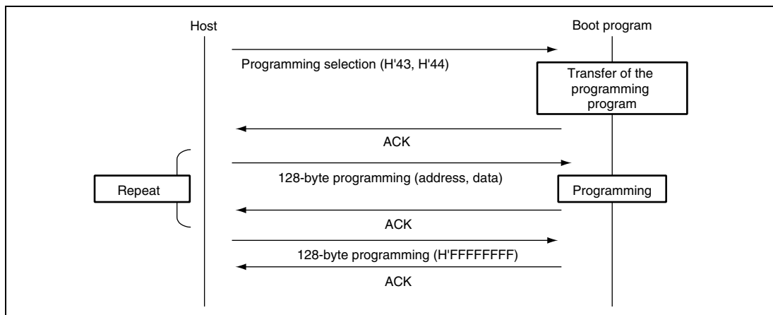
Figure 20.24 Programming Sequence
