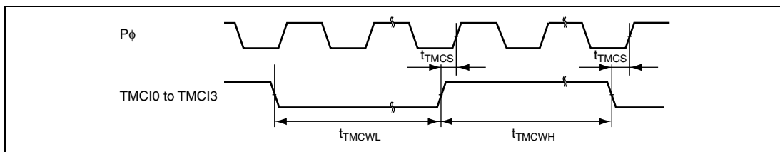
Figure 24.31 8-Bit Timer Clock Input Timing
