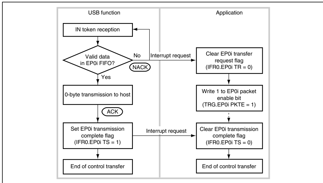
Figure 15.14 Status Stage (Control-Out) Operation
