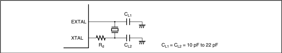
Figure 21.2 Connection of Crystal Resonator (Example)
