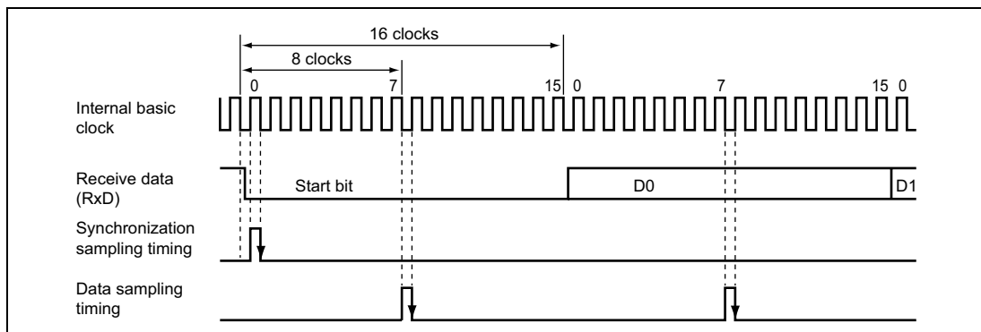
Figure 14.6 Receive Data Sampling Timing in Asynchronous Mode
