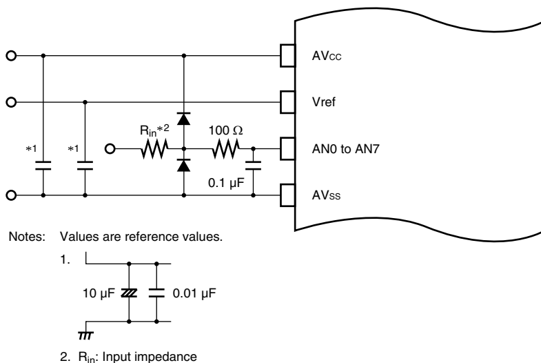
Figure 17.9 Example of Analog Input Protection Circuit
