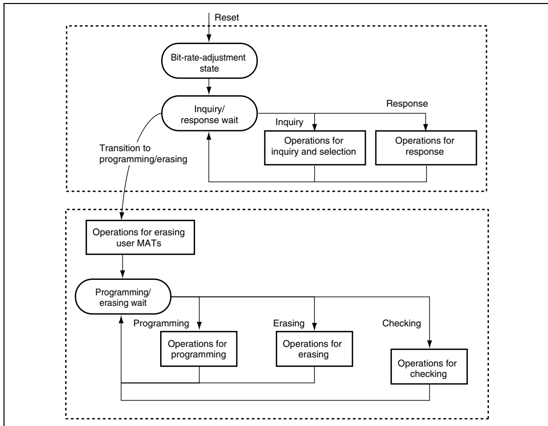
Figure 20.20 Boot Program States
