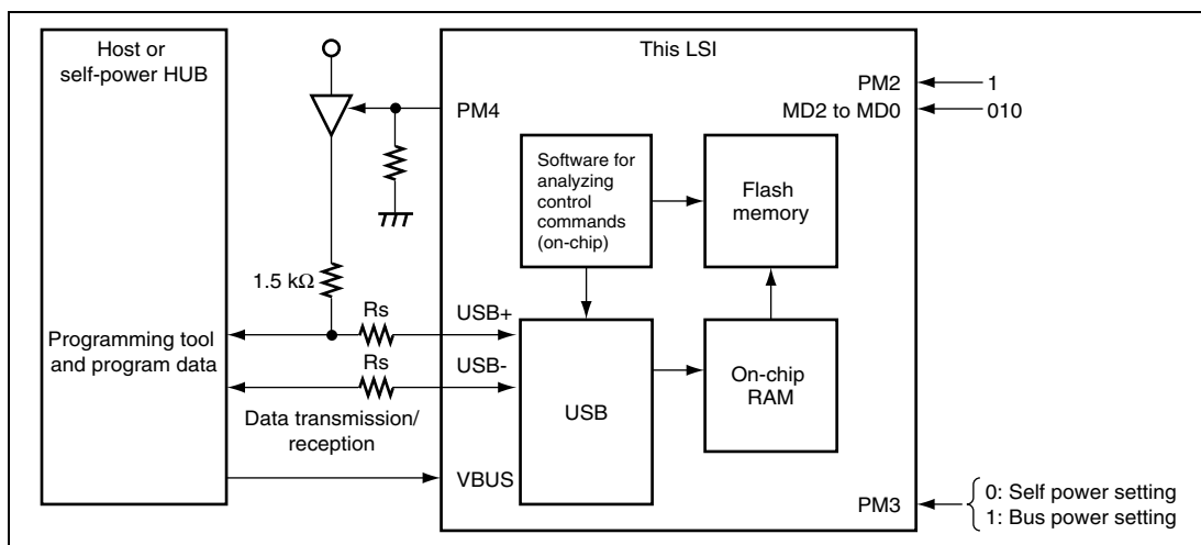
Figure 20.9 System Configuration in USB Boot Mode
