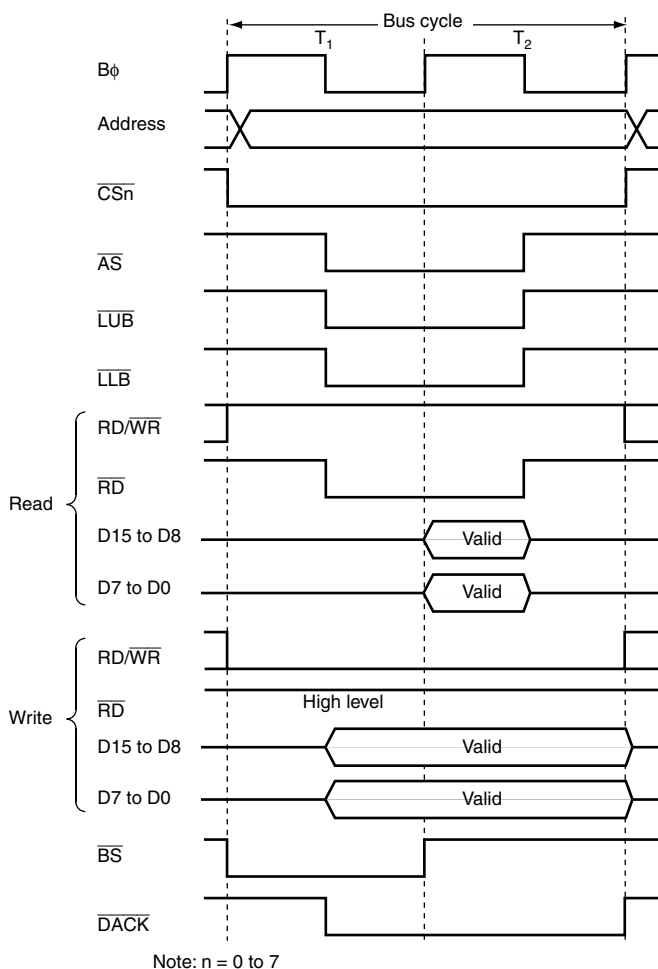
Figure 6.24 16-Bit 2-State Access Space Bus Timing
