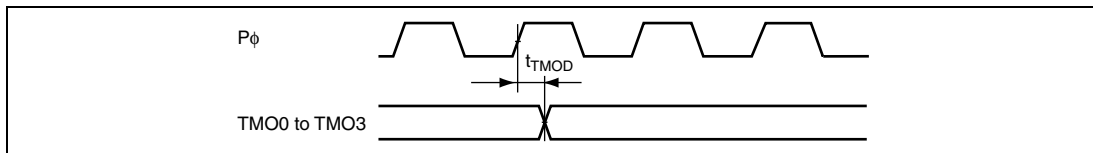
Figure 24.29 8-Bit Timer Output Timing
