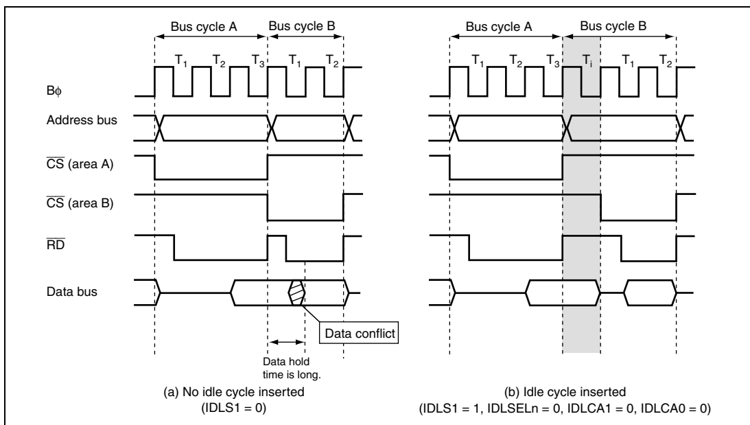
Figure 6.37 Example of Idle Cycle Operation (Consecutive Reads in Different Areas)
