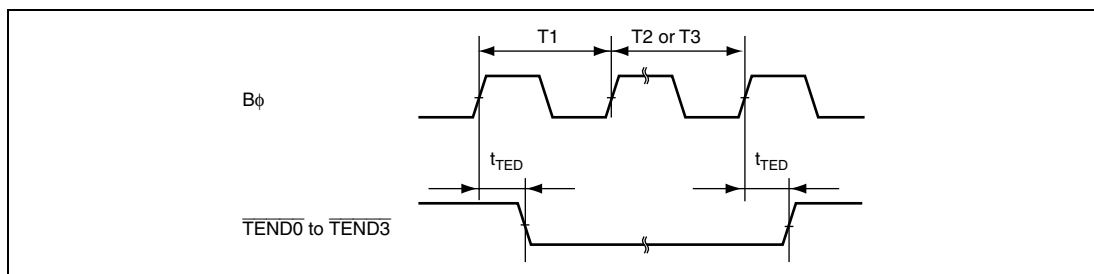
Figure 24.22 DMAC ( \overline{TEND} ) Output Timing
