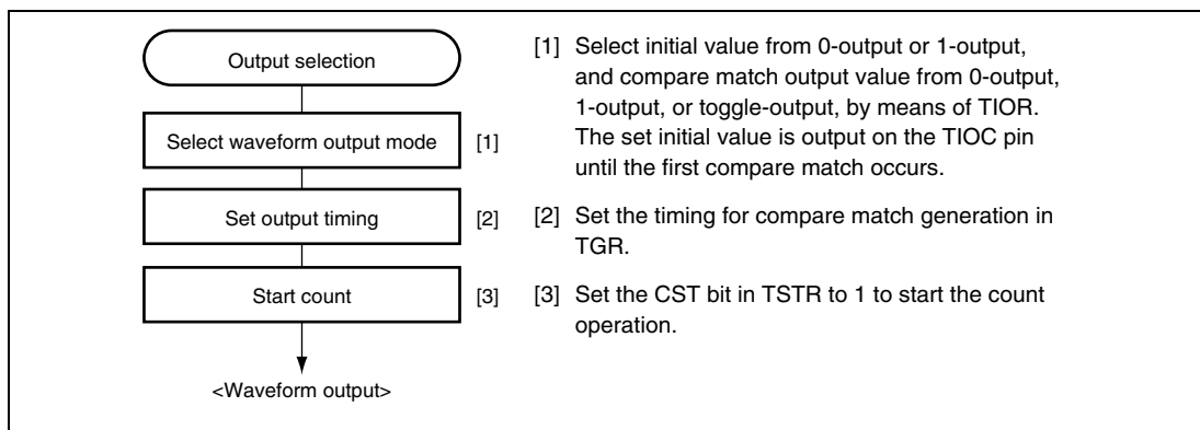
Figure 10.5 Example of Setting Procedure for Waveform Output by Compare Match
