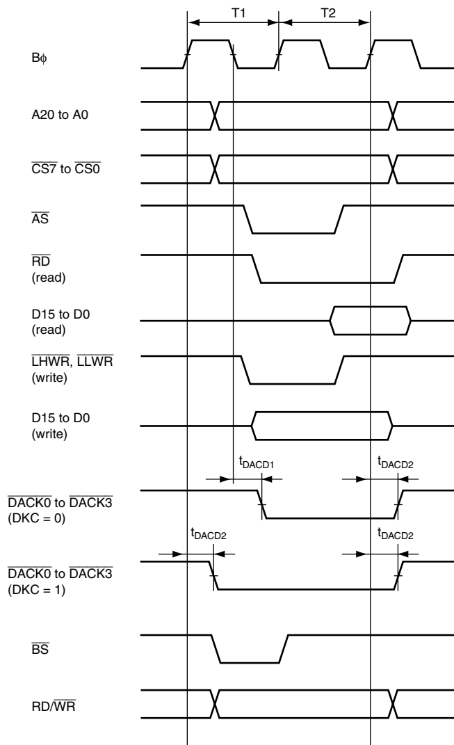
Figure 24.23 DMAC Single-Address Transfer Timing: Two-State Access
