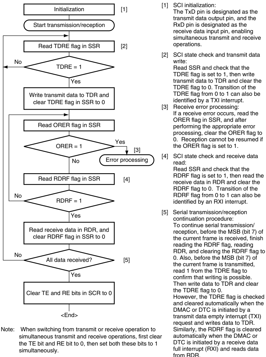
Figure 14.23 Sample Flowchart of Simultaneous Serial Transmission and Reception
