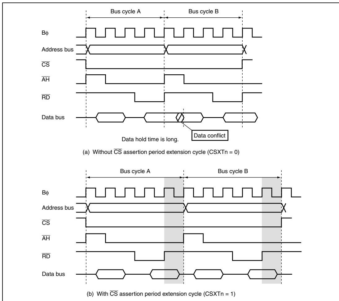
Figure 6.35 Consecutive Read Accesses to Same Area (Address/Data Multiplexed I/O Space)
