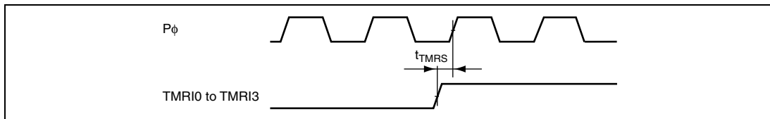
Figure 24.30 8-Bit Timer Reset Input Timing
