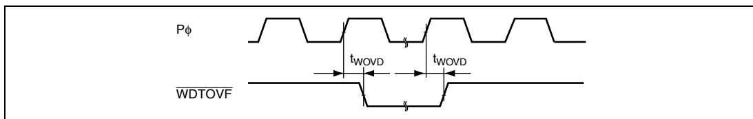
Figure 24.32 WDT Output Timing
