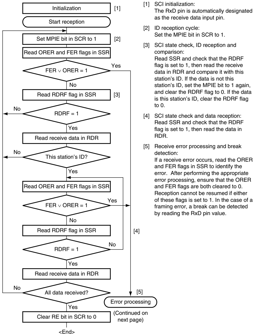
Figure 14.16 Sample Multiprocessor Serial Reception Flowchart (1)
