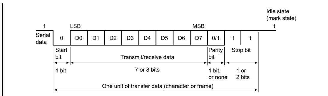
Figure 14.5 Data Format in Asynchronous Communication (Example with 8-Bit Data, Parity, Two Stop Bits)
