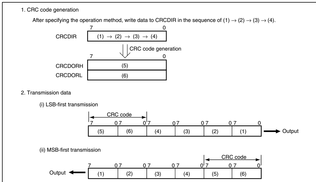
Figure 14.48 LSB-First and MSB-First Transmit Data
