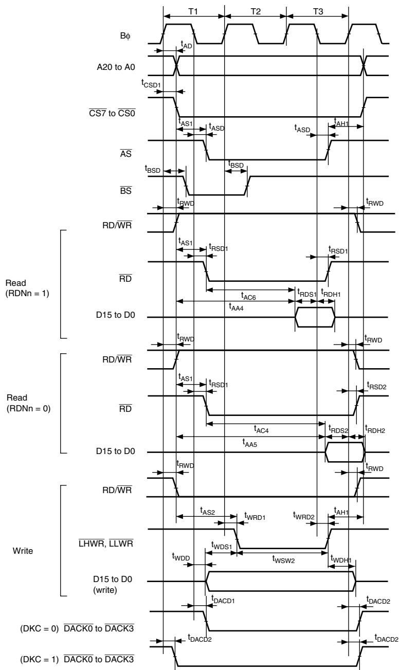
Figure 24.9 Basic Bus Timing: Three-State Access
