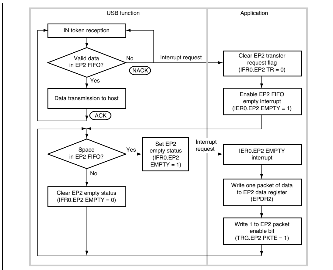
Figure 15.16 EP2 Bulk-In Transfer Operation
