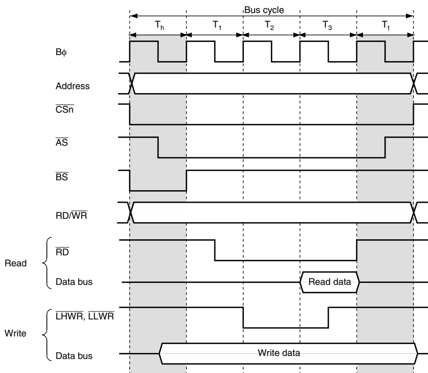
Figure 6.3 \overline{\text{CS}} and Address Assertion Period Extension (Example of Basic Bus Interface, 3-State Access Space, and RDNn = 0)
