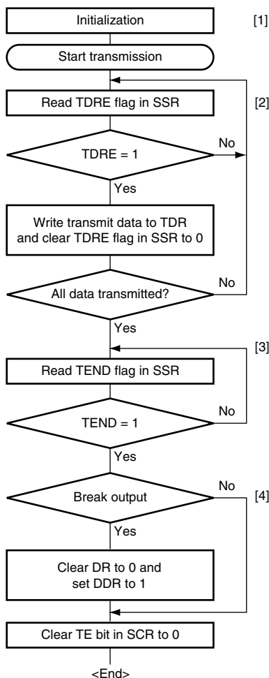
Figure 14.10 Example of Serial Transmission Flowchart
