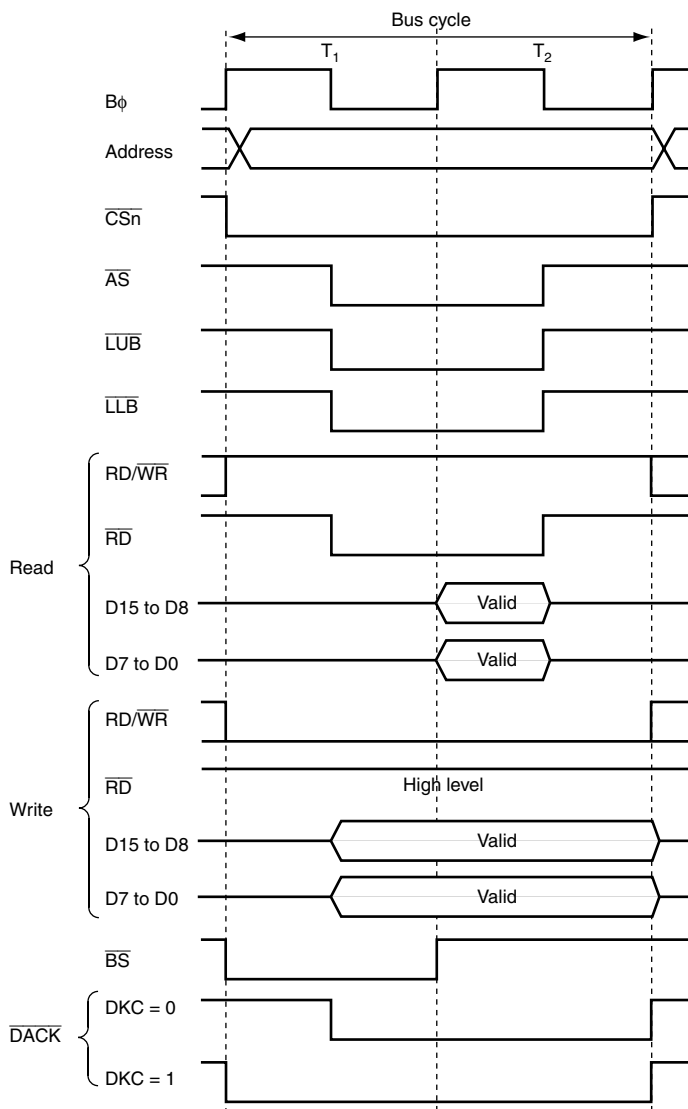
Figure 6.27 \overline{DACK} Signal Output Timing
