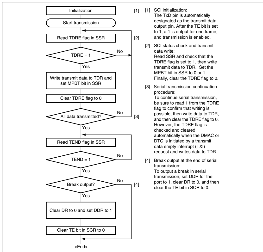
Figure 14.14 Sample Multiprocessor Serial Transmission Flowchart
