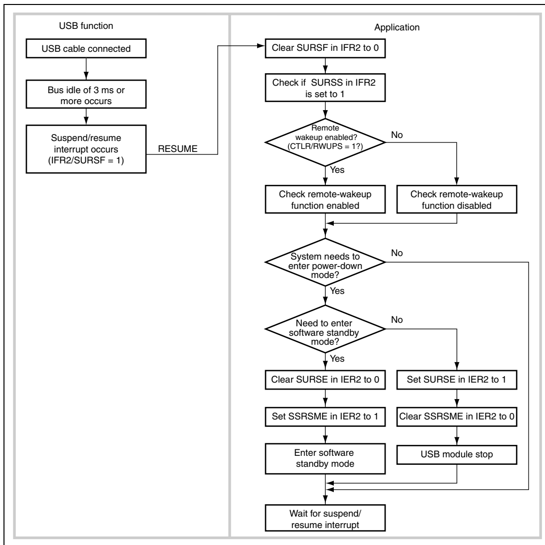
Figure 15.4 Suspend Operation
