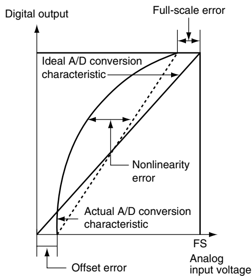
Figure 17.7 A/D Conversion Accuracy Definitions
