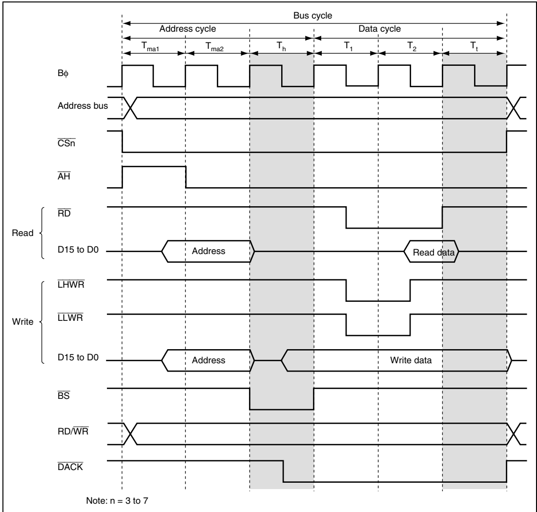
Figure 6.34 Chip Select ( \overline{\text{CS}} ) Assertion Period Extension Timing in Data Cycle
