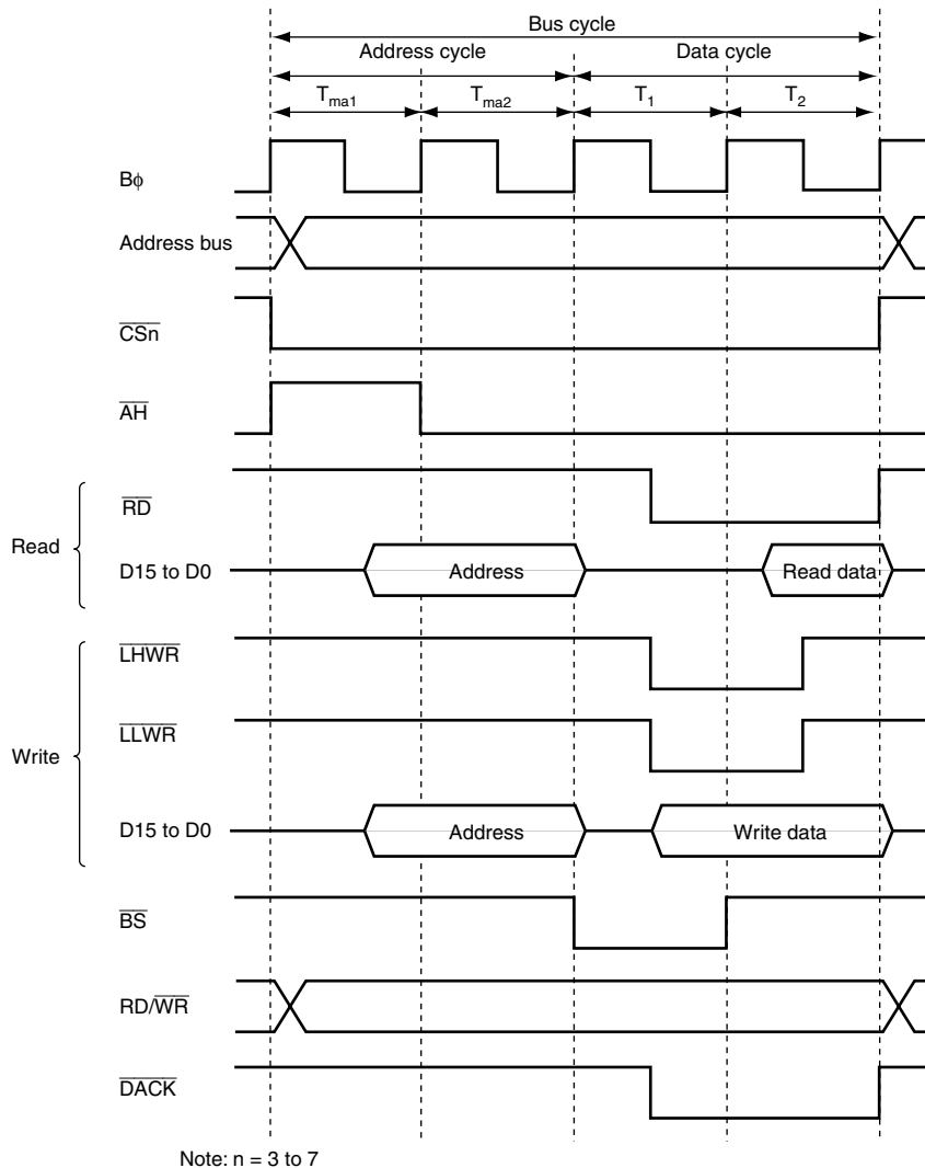
Figure 6.31 16-Bit Access Space Access Timing (ABWHn = 0, ABWLn = 1)
