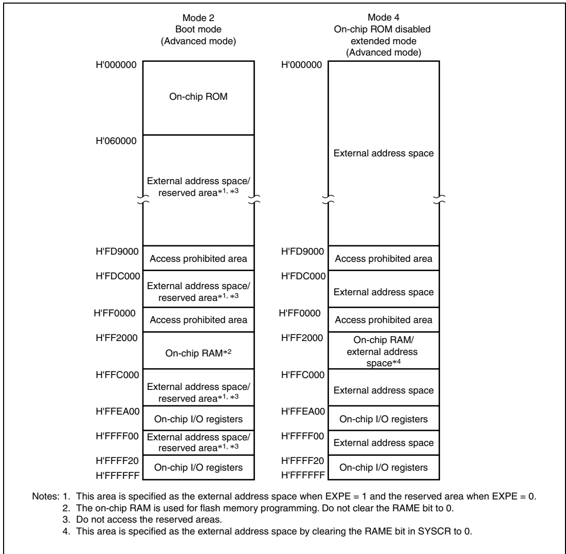
Figure 3.1 Address Map (1) in each Operating Mode of H8SX/1653
