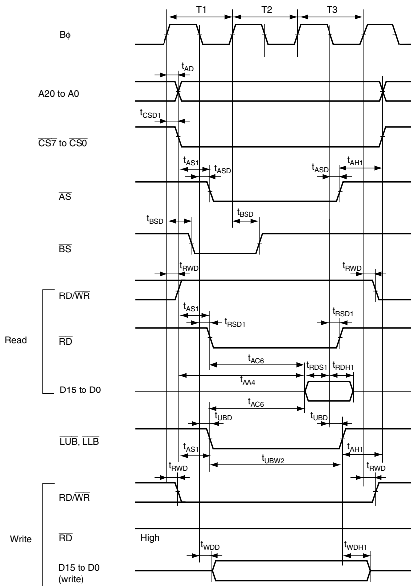
Figure 24.14 Byte Control SRAM: Three-State Read/Write Access
