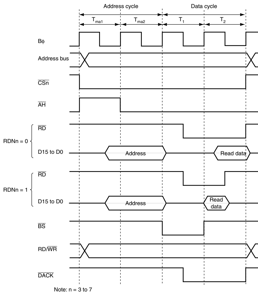
Figure 6.33 Read Strobe Timing
