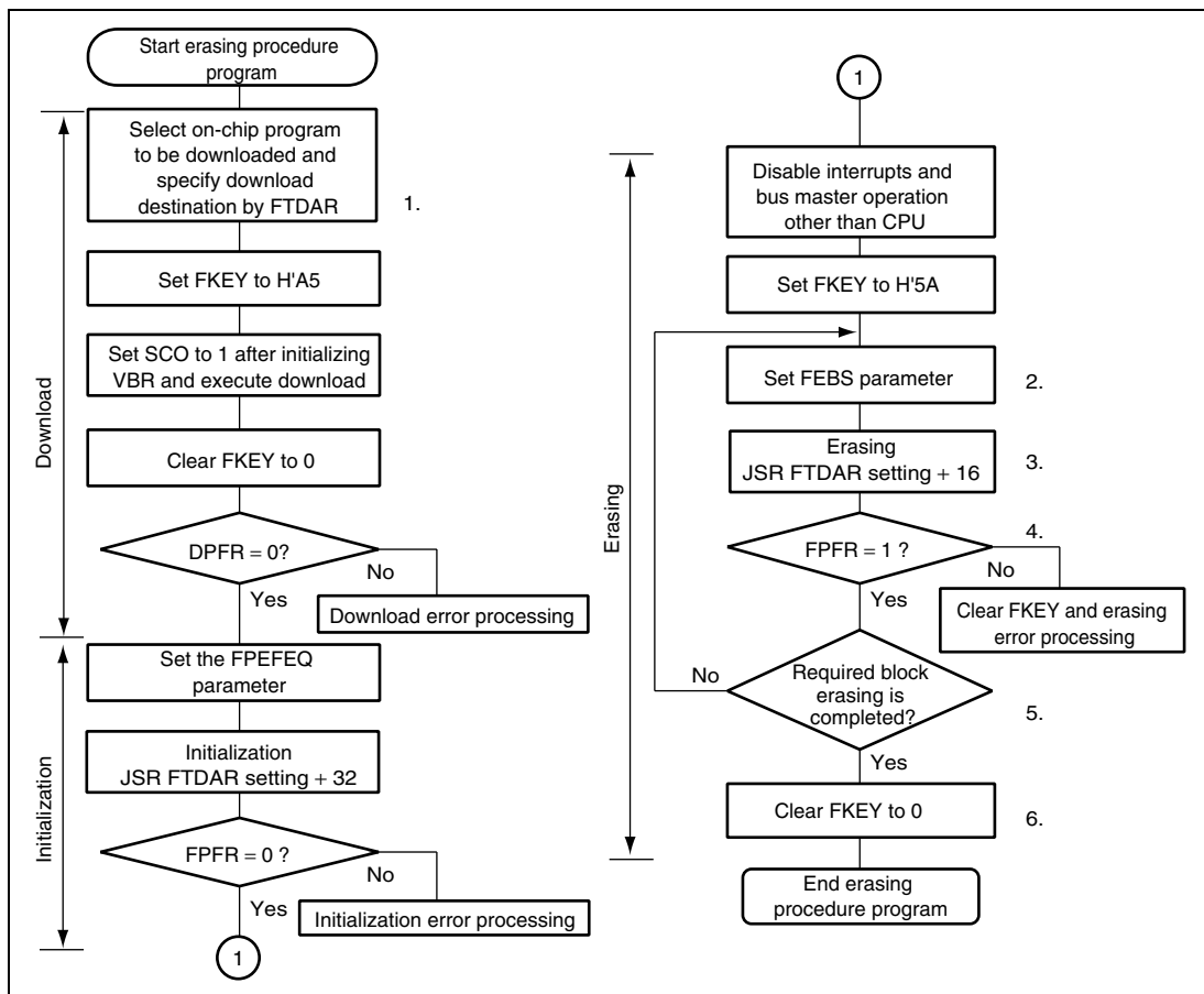
Figure 20.14 Erasing Procedure in User Program Mode
