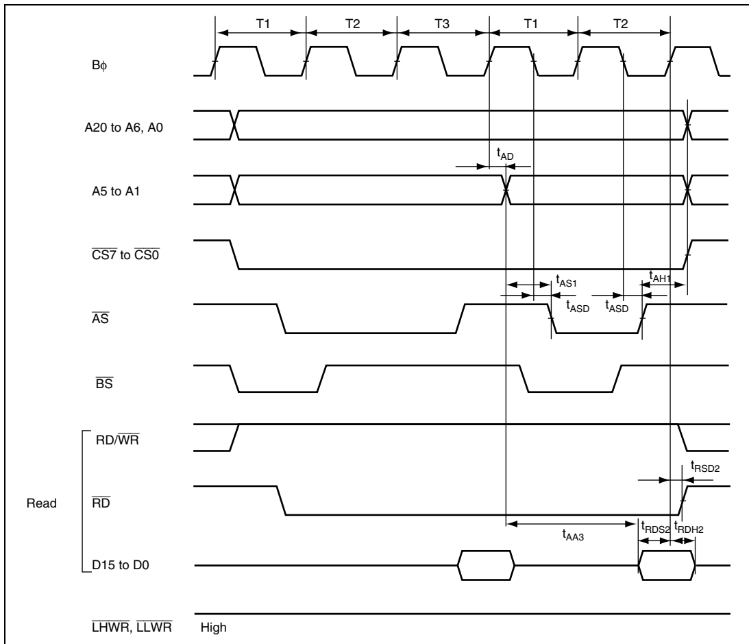
Figure 24.16 Burst ROM Access Timing: Two-State Burst Access
