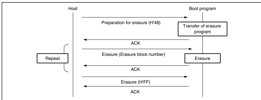
Figure 20.25 Erasure Sequence
