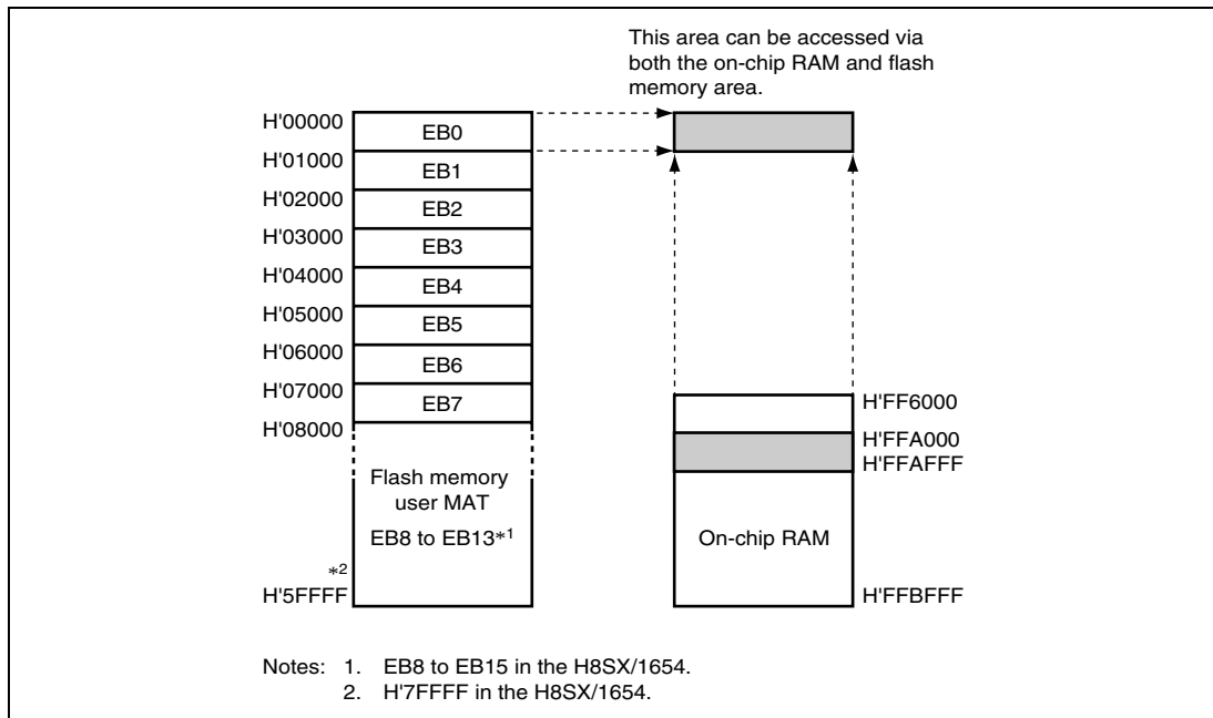
Figure 20.18 Address Map of Overlaid RAM Area (H8SX/1653)
