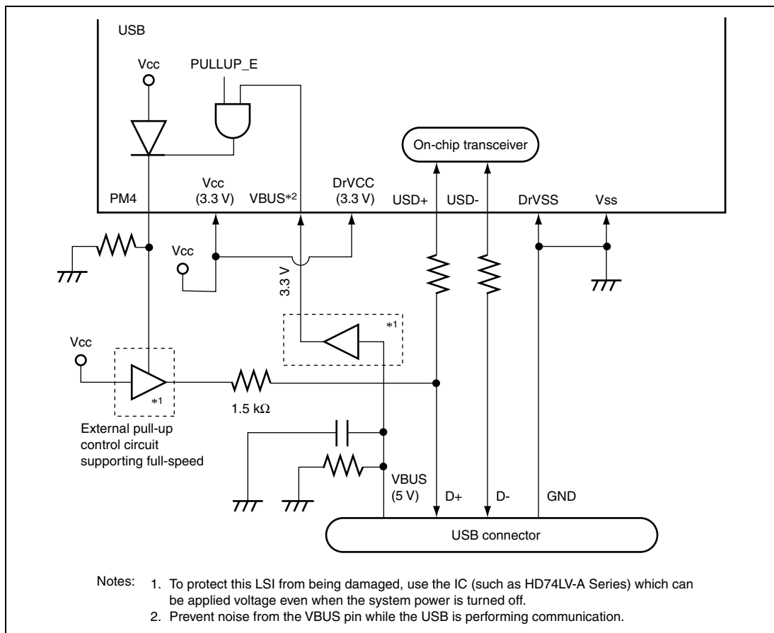
Figure 15.23 Example of Circuitry in Self Power Mode
