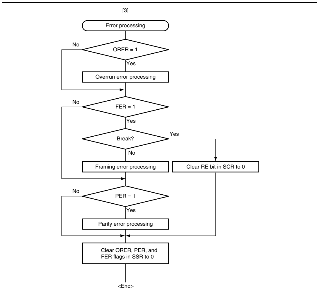
Figure 14.12 Sample Serial Reception Flowchart (2)
