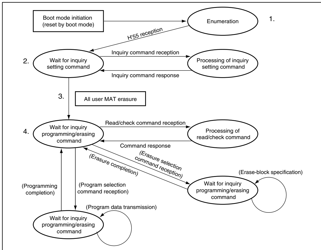
Figure 20.10 USB Boot Mode State Transition Diagram
