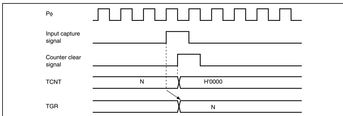
Figure 10.35 Counter Clear Timing (Input Capture)
