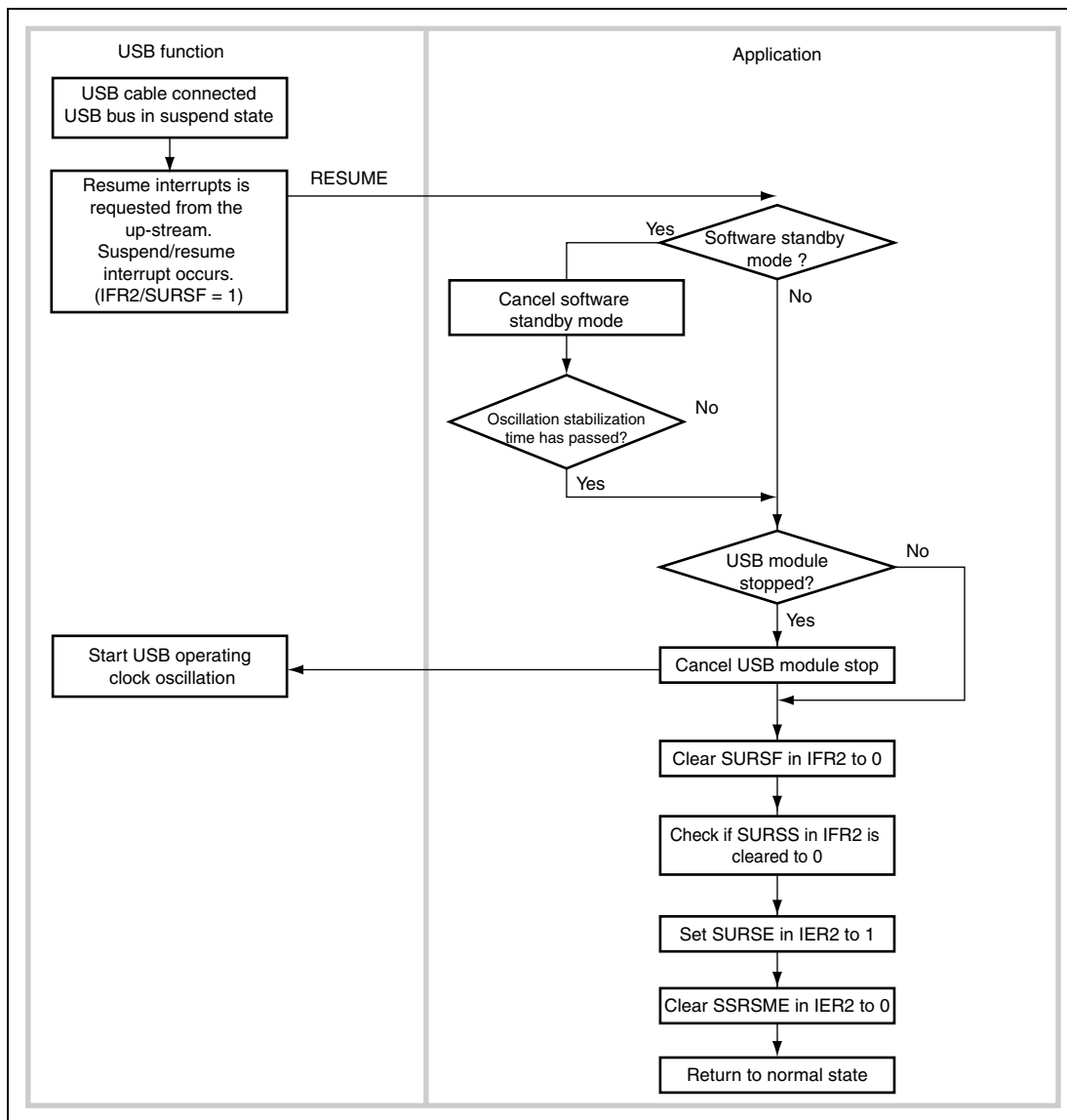
Figure 15.5 Resume Operation from Up-Stream
