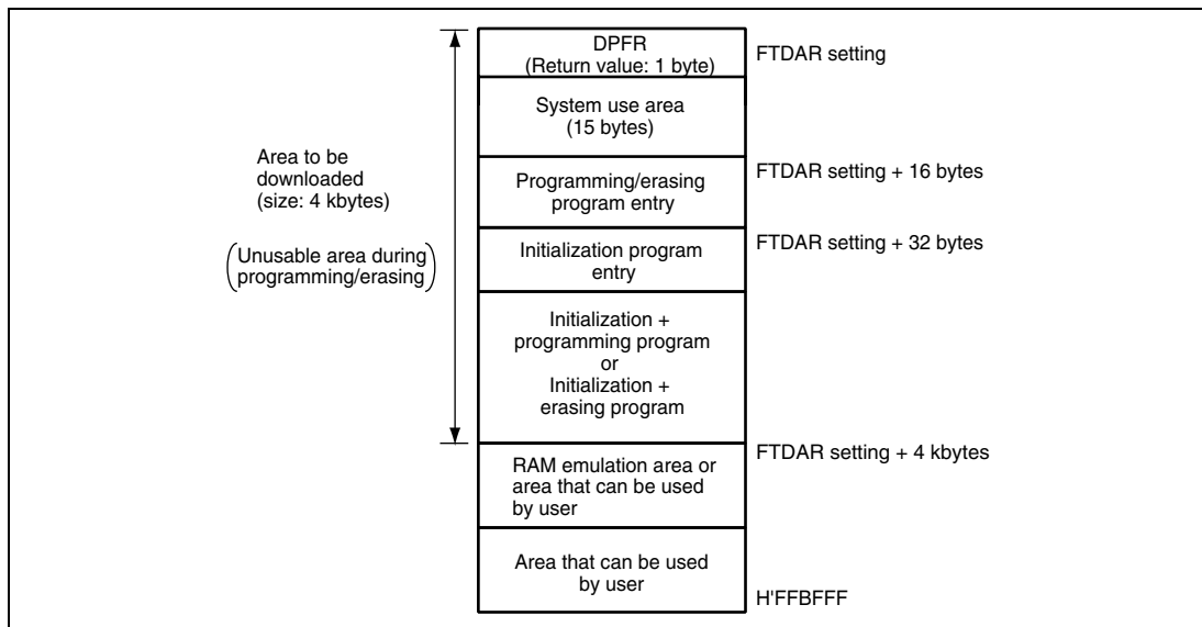
Figure 20.12 RAM Map when Programming/Erasing is Executed
