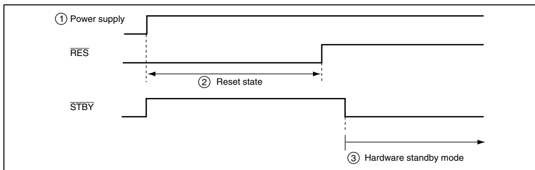
Figure 22.4 Timing Sequence at Power-On
