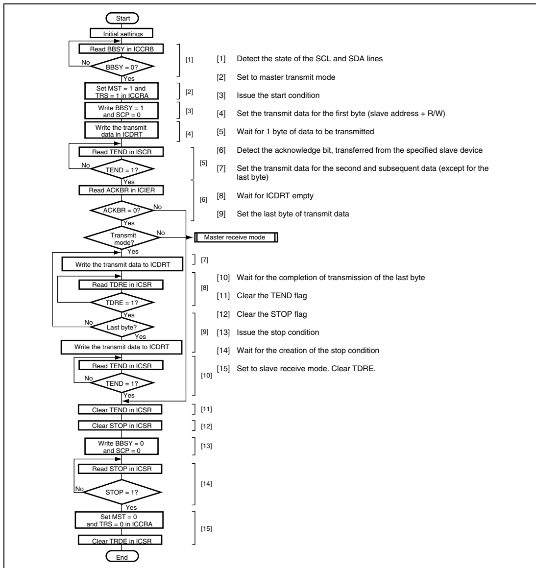
Figure 16.14 Sample Flowchart of Master Transmit Mode
