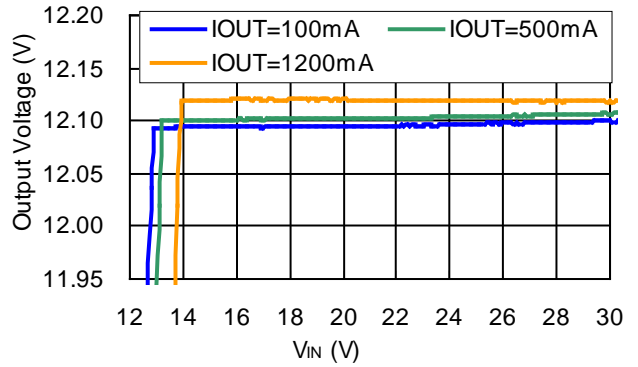
R1245x00xA/R1245x00xB
