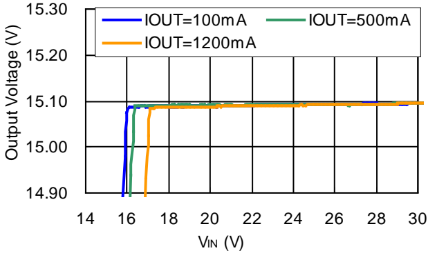
R1245x00xC/R1245x00xD
