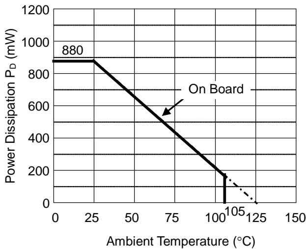
Power Dissipation
