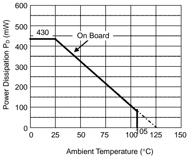
Power Dissipation
