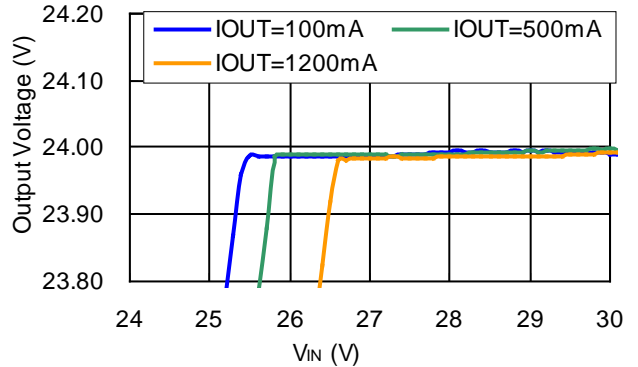
R1245x00xC/R1245x00xD
