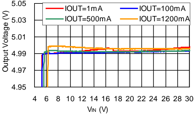
R1245x00xA/R1245x00xB
