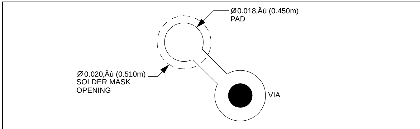
Figure 87: Recommended PCB layout for BGA landing pad for 23x23 mm 2 package
