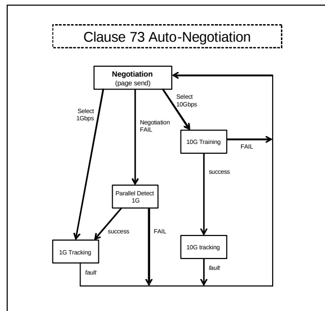
Figure 13: Simplified Auto-Negotiation State Diagram
