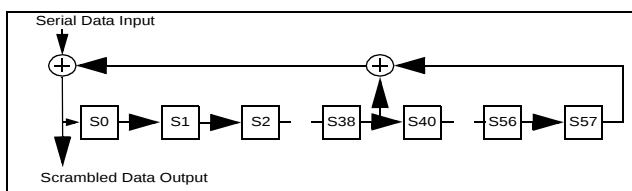
Figure 7: Transmit Scrambler
