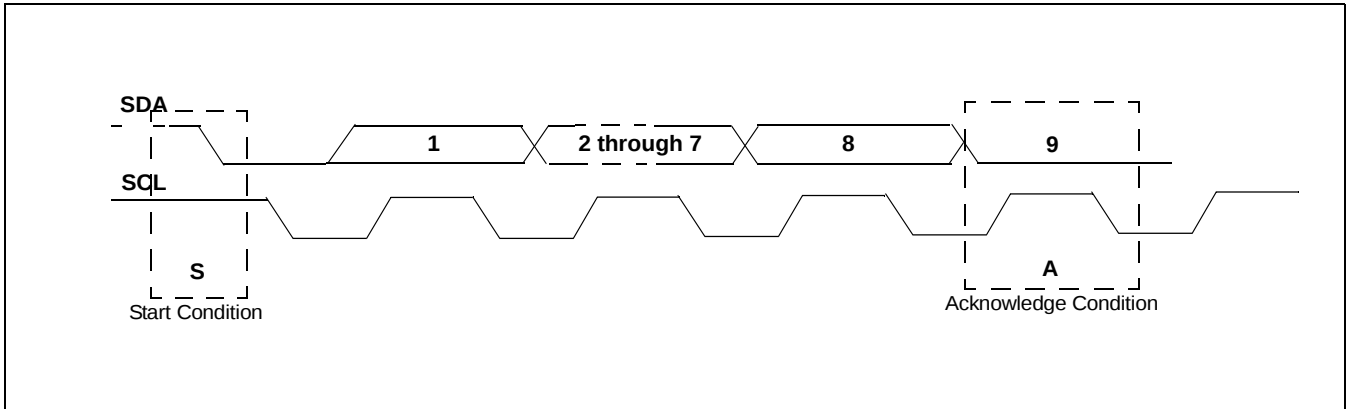
Figure 53: Acknowledge Condition
