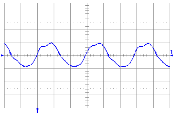
Figure 20. Output voltage ripple (20 mV/div.) at full rated load current into a resistive load with C_o = 10\ \mu\text{F} tantalum + 1 \mu\text{F} ceramic and V_{in} = 48\text{ V} . Time scale: 1 \mu\text{s} /div.
