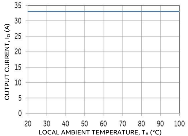
Figure 24. Output Current Derating for the Base Plate QBW033A0B-H at 48V in in a Cold wall application; Local Internal Air Temperature near module=80°C; VOUT setting anywhere from 6.0V to 12.0V
