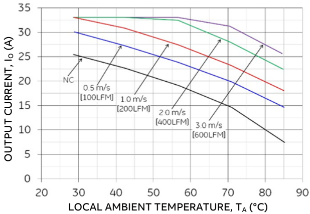
Figure 20. Output Current Derating for the Base plate QBW033A0B-H at 48V in with Transverse airflow from V_{in}(-) to V_{in}(+)
