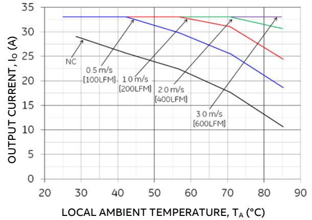
Figure 22. Output Current Derating for the Base plate QBW033A0B-H at 48V in with 0.5" heatsink and Transverse airflow from V_{in}(-) to V_{in}(+)
