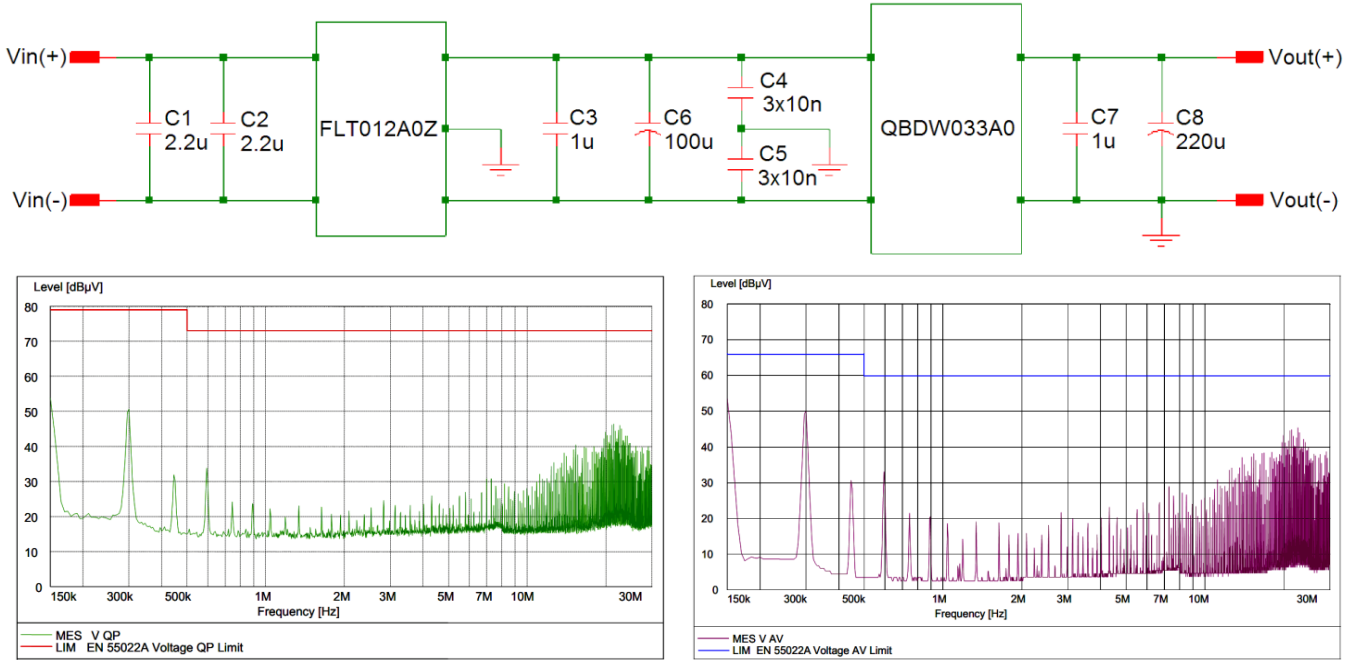
Figure 25. EMC Consideration
