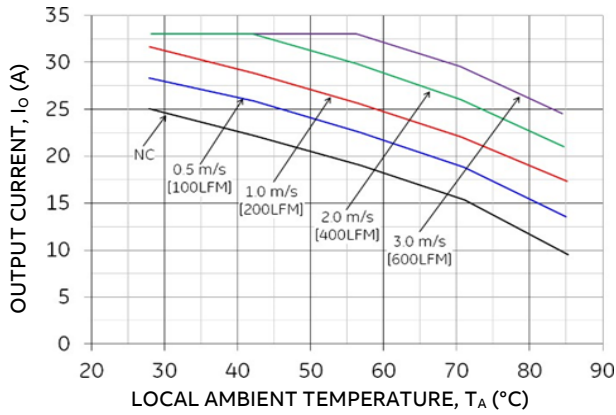
Figure 19. Output Current Derating for the Open Fram QBW033A0B at 48V in with Transverse airflow from V_{in}(-) to V_{in}(+)
