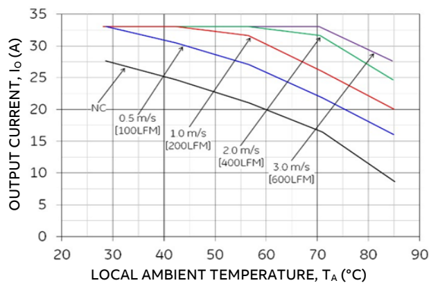
Figure 21. Output Current Derating for the Base plate QBW033A0B-H at 48V in with 0.25" heatsink and Transverse airflow from V_{in}(-) to V_{in}(+)
