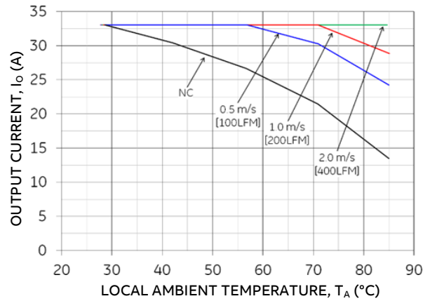
Figure 23. Output Current Derating for the Base plate QBW033A0B-H at 48V in with 1.0" heatsink and Transverse airflow from V_{in}(-) to V_{in}(+)
