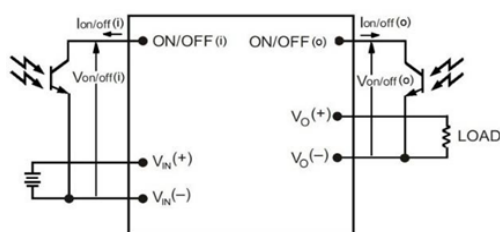
Figure 14. Remote On/Off Implementa-
