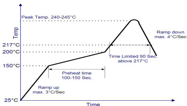
Figure 24. Recommended linear reflow profile using Sn/Ag/Cu solder.
