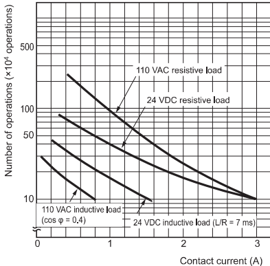
Endurance Curve MY4H
