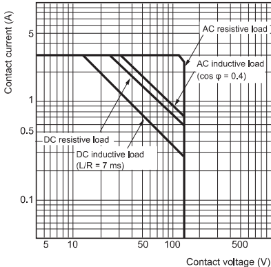
Maximum Switching Capacity MY4(Z)H
