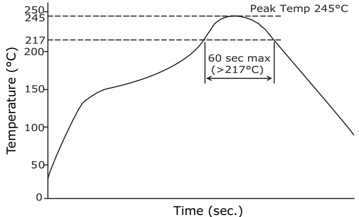
Reflow Soldering Profile (SMT models)
