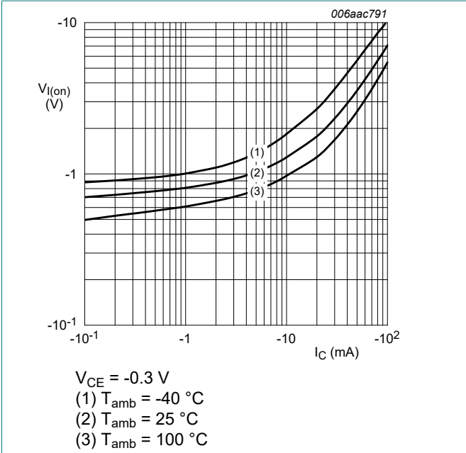
Fig. 11. TR2 (PNP): On-state input voltage as a function of collector current; typical values
