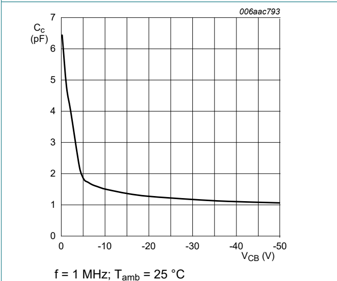
Fig. 13. TR2 (PNP): Collector capacitance as a function of collector-base voltage; typical values
