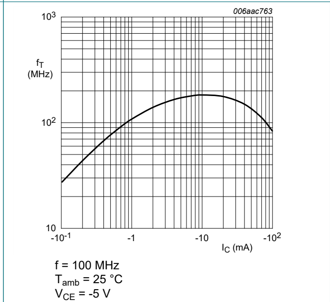
Fig. 14. TR2 (PNP): Transition frequency as a function of collector current; typical values of built-in transistor
