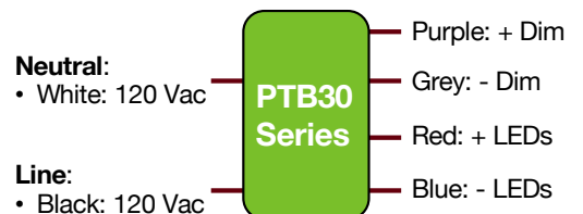
Wiring Diagram
