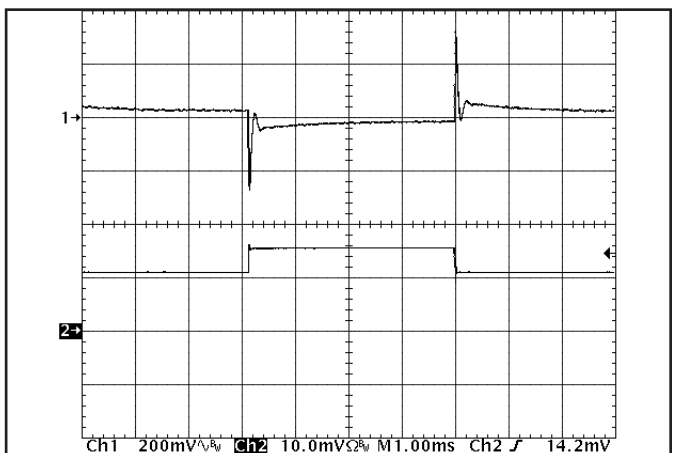
Figure 12: Output voltage response to step-change in load current (50%-75%-50% of I_{out(max)} ; dI/dt = 5A/\mu s ). Load cap: 470 \mu F , 15 m \Omega ESR tantalum cap and 1 \mu F ceramic cap. Top trace: V_{out} (200mV/div), Bottom trace: I_{out} (20A/div).
