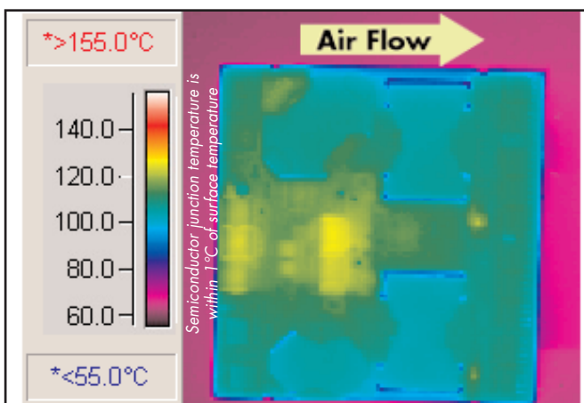
Figure 6: Thermal plot of converter at 39 amp load current (195 Watts) with 55°C air flowing at the rate of 200 LFM. Air is flowing across the converter from input to output (nominal input voltage).
