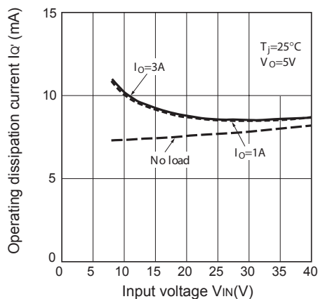
Fig.6 Operating Dissipation Current vs. Input Voltage
