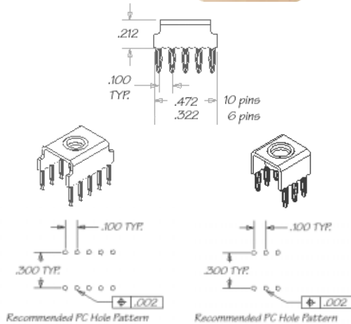
Recommended PC Hole Pattern
