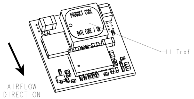
Figure 47. Preferred airflow direction and location of hot-spot of the module ( T_{ref} ).
