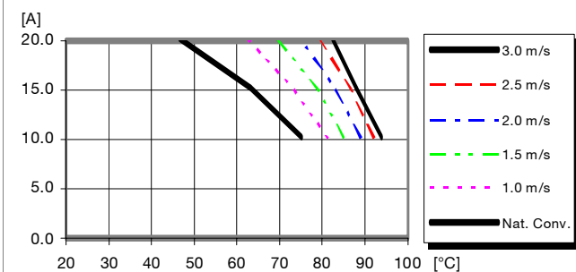
Available load current vs. ambient air temperature and airflow at V_i = 53\text{ V} . See Thermal Consideration section.
