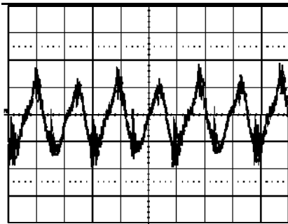
Output voltage ripple at: T_{ref} = +25^{\circ}\text{C} , V_i = 53\text{ V} , I_o = 25\text{ A} resistive load. Trace: output voltage (20mV/div.). Time scale: (2 μs/div.).
