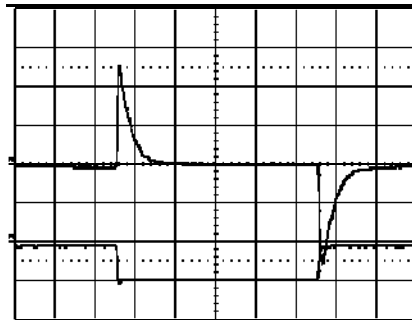
Output voltage response to load current step- Trace: output voltage (100mV/div.). change (15-30-15 A) at: T_{ref} = +25^\circ\text{C} , V_i = 53\text{ V} . Time scale: (0.1 ms/div.).
