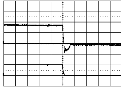
Shut-down enabled by disconnecting V_i at: T_{ref} = +25^\circ\text{C} , V_i = 53\text{ V} , I_o = 80\text{ A} resistive load. Top trace: output voltage (1 V/div.). Bottom trace: input voltage (50 V/div.). Time scale: (0.5 ms/div.).
