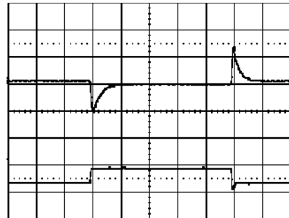
Output voltage response to load current step- Trace: output voltage (200mV/div.). change (20-40-20 A) at: T_{ref} = +25^\circ\text{C} , V_i = 53\text{ V} . Time scale: (0.1 ms/div.).
