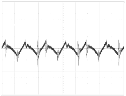
Output voltage ripple at: T_{ref} = +25^{\circ}\text{C} , V_i = 53\text{ V} , I_o = 30\text{ A} resistive load. Trace: output voltage (50mV/div.), Time scale: (2 \mu\text{s} /div.).
