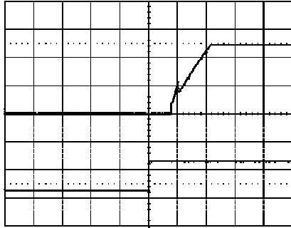
Start-up enabled by connecting V_i at: T_{ref} = +25^{\circ}\text{C} , V_i = 53\text{ V} , I_o = 30\text{ A} resistive load. Top trace: input voltage (50 V/div.), Bottom trace: output voltage (1 V/div.), Time scale: (10 ms/div.).
