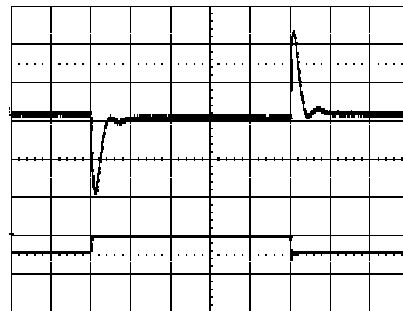
Output voltage response to load current step- change (7.5-15-7.5 A) at: T_{ref} = +25^{\circ}\text{C} , V_i = 53\text{ V} . Trace: output voltage (100mV/div.), Time scale: (0.1 ms/div.).
