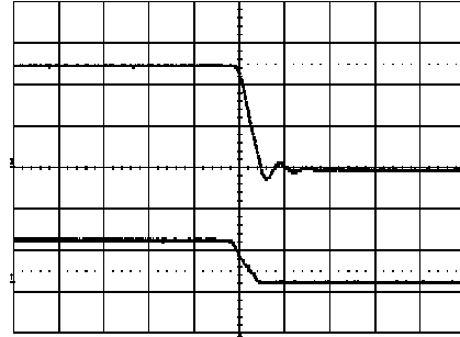
Shut-down enabled by disconnecting V_i at: T_{ref} = +25^{\circ}\text{C} , V_i = 53\text{ V} , I_o = 30\text{ A} resistive load. Top trace: output voltage (1 V/div.), Bottom trace: input voltage (50 V/div.), Time scale: (0.2 ms/div.).
