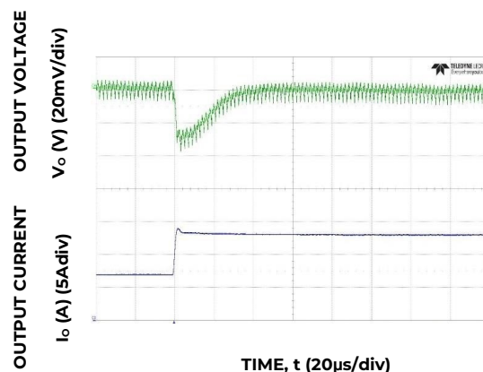
Figure 16. Transient Response to Dynamic Load Change from 50% to 100% at 12V in , C_{out}=8x47\mu F+2x330\mu F C_{Tune}=1.8nF , R_{Tune}=300\Omega
