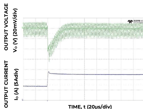
Figure 22. Transient Response to Dynamic Load Change from 50% to 100% at 12V in , C_{out}=4x47\mu F+1x330\mu F , C_{Tune}=1.2nF , R_{Tune}=300\Omega
