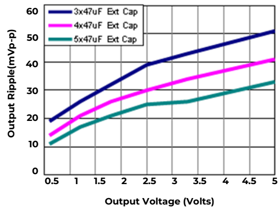
Figure 38. Output ripple voltage for various output voltages with external 3x47 \mu F, 4x47 \mu F or 5x47 \mu F ceramic capacitors at the output (14A load). Input voltage is 12V.
