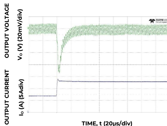
Figure 28 Transient Response to Dynamic Load Change from 50% to 100% at 12V in , C_{out}=8 \times 47\mu\text{F} , C_{Tune}=1.2\text{nF} , R_{Tune}=300\Omega
