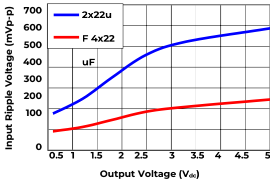
Figure 37. Input ripple voltage for various output voltages with 2x22 \mu F or 4x22 \mu F ceramic capacitors at the input (14A load). Input voltage is 12V.
