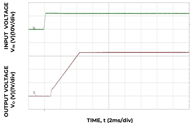
Figure 30. Typical Start-up Using Input Voltage ( V_{IN}=12\text{V} , I_o=I_{o,max} ).
