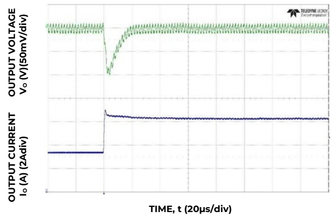
Figure 34. Transient Response to Dynamic Load Change from 50% to 100% at 12V in , C out = 3x47μF, C Tune =1.8 nF, R Tune =300Ω
