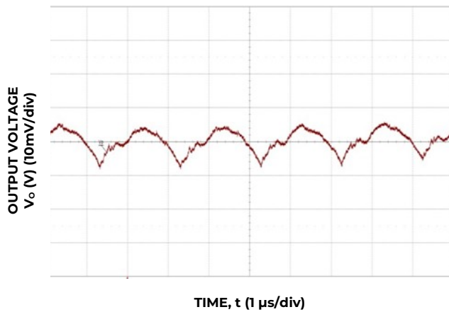
Figure 9. Typical output ripple ( C_o=3 \times 22 \mu F ceramic, V_{IN} = 12V , I_o = I_{o,max} ).
