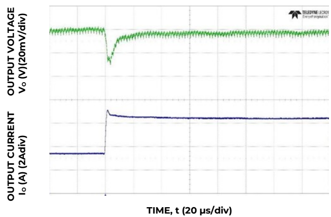
Figure 10. Transient Response to Dynamic Load Change from 50% to 100% at 12V in , C_{out} = 6 \times 47 \mu F + 1 \times 330 \mu F , C_{Tune} = 12 nF , R_{Tune} = 300 \Omega
