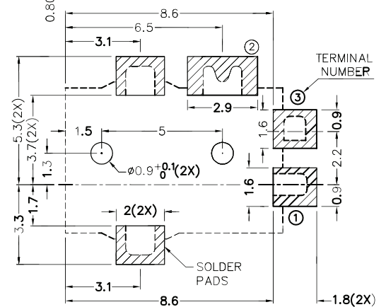
RECOMMENDED PCB LAYOUT TOLERANCE: \pm 0.05 (TOP VIEW)
