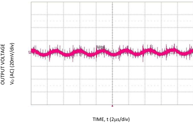
Fig 12: 3.3V Ripple
