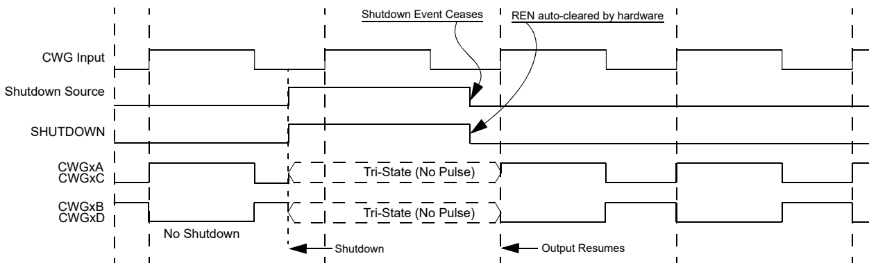
Figure 31-16. Shutdown Functionality, Auto-Restart Enabled ( REN = 1 , LSAC = 'b01 , LSBD = 'b01 )
