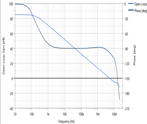
Figure 49-9. Open Loop Gain at V_{CM} = V_{DD}/2 over V_{DD} and Temperature
