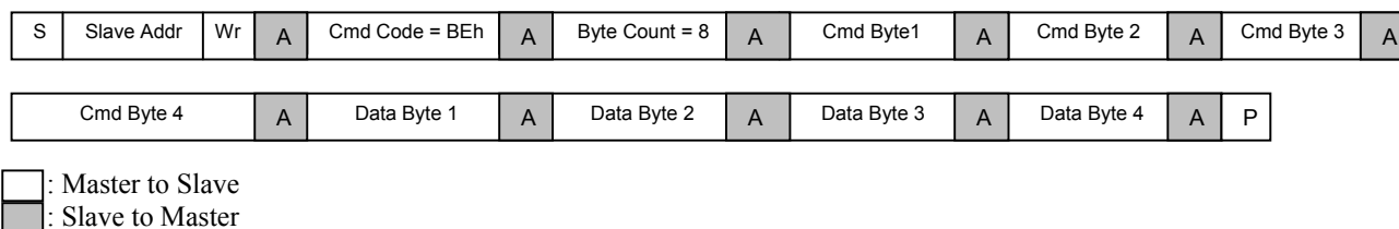
Figure 7-2 SMBus Block Write Command Format, to Write to a PI7C9X2G608GP Register without PEC
