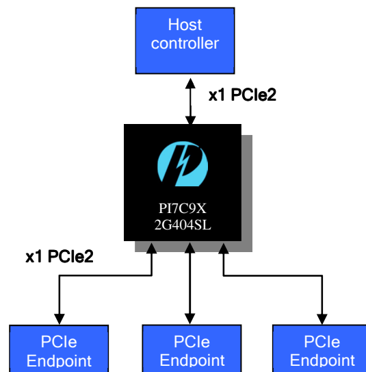
PI7C9X2G404SL – Application Example
