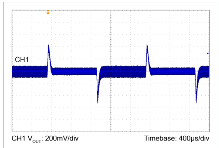
Figure 28 — 24V_{IN} to 36V_{OUT} , C_{OUT} = 8 \times 10\mu\text{F} Ceramic 1.5A to 3.0A Load Step, 0.1\text{A}/\mu\text{s}
