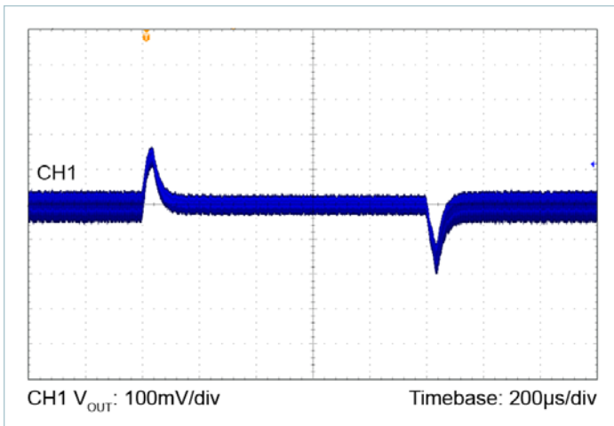
Figure 25 — 24V_{IN} to 12V_{OUT} , C_{OUT} = 8 \times 10\mu\text{F} Ceramic 3.38A to 6.75A Load Step, 0.1\text{A}/\mu\text{s}
