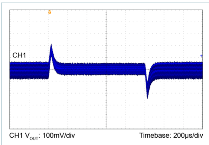
Figure 26 — 24V_{IN} to 24V_{OUT} , C_{OUT} = 8 \times 10\mu\text{F} Ceramic 2.5A to 5.0A Load Step, 0.1\text{A}/\mu\text{s}
