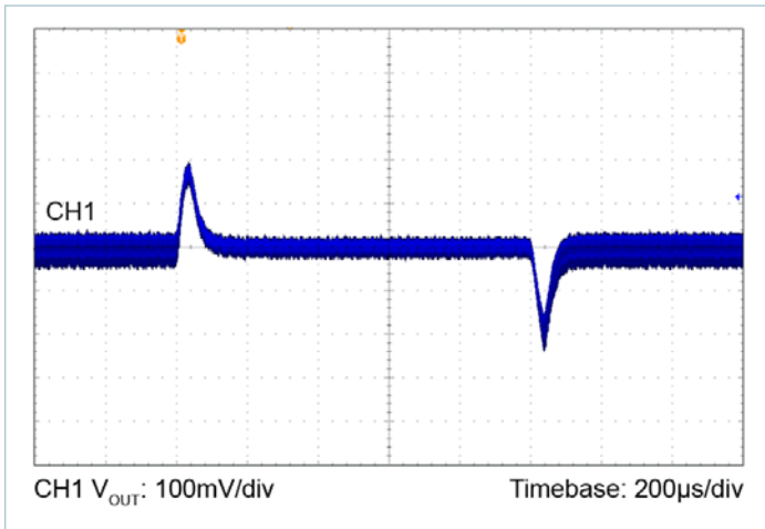
Figure 24 — 24V_{IN} to 10V_{OUT} , C_{OUT} = 8 \times 10\mu\text{F} Ceramic 3.5A to 7.0A Load Step, 0.1\text{A}/\mu\text{s}
