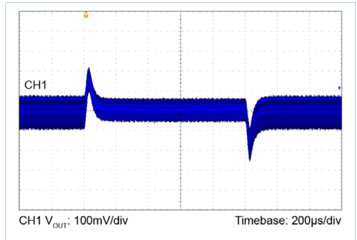
Figure 27 — 24V_{IN} to 28V_{OUT} , C_{OUT} = 8 \times 10\mu\text{F} Ceramic 2.25A to 4.5A Load Step, 0.1\text{A}/\mu\text{s}
