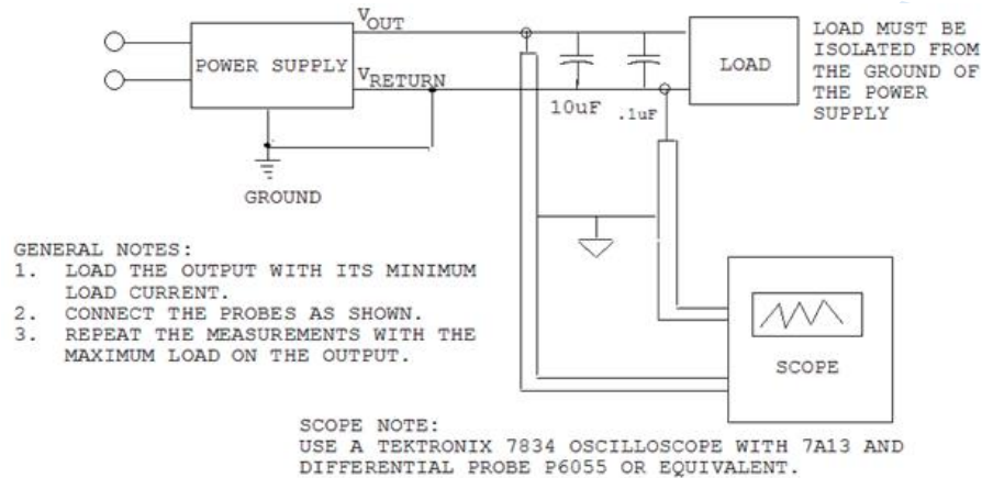
Figure 5. Output ripple test setup
