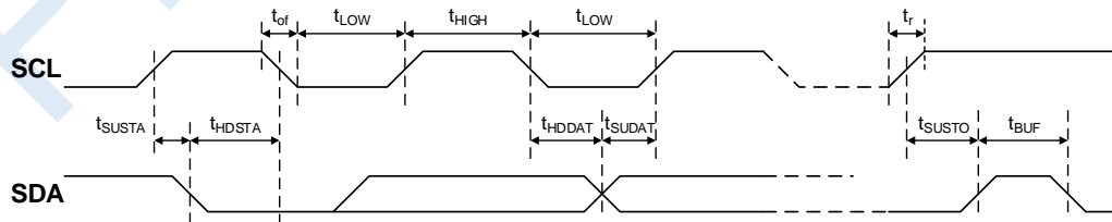
Figure 16. I2C / SMBus Timing
