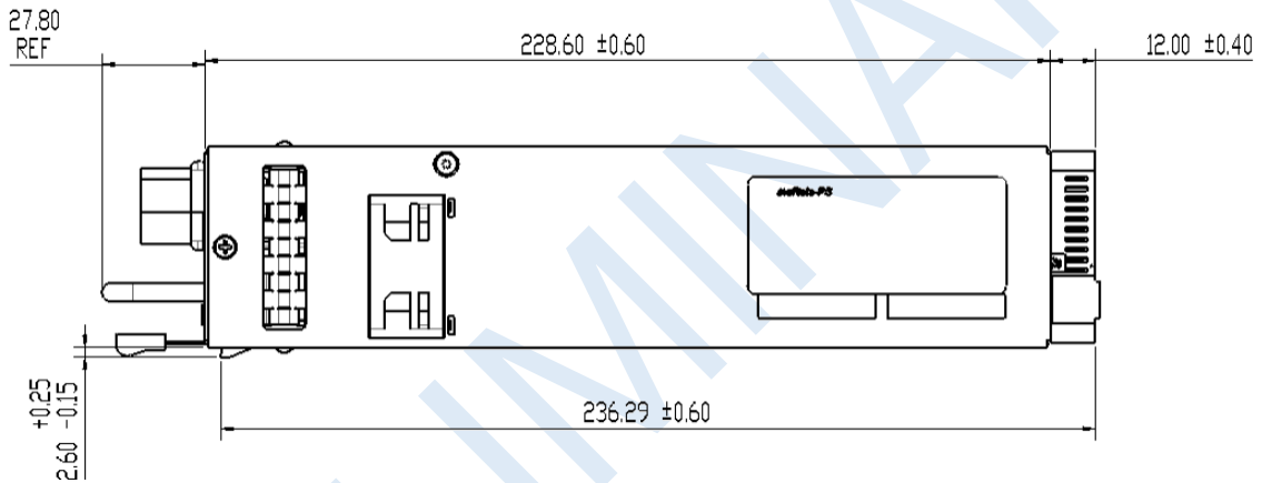
Figure 21. Top View
