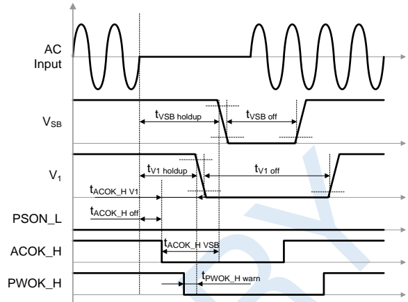
Figure 12. AC long dips
