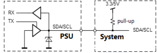
Figure 15. Physical layer of communication interface
