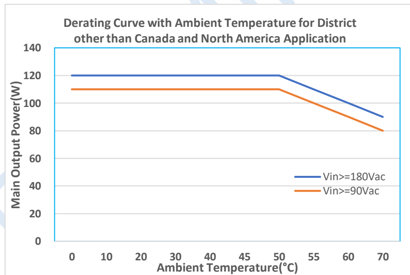
Figure 6c. OCP Derating Curve with Ambient Temperature
