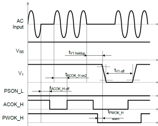
Figure 11. AC short dips
