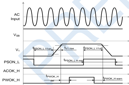
Figure 13. PSON_L and PWOK_H turn-on/off timing
