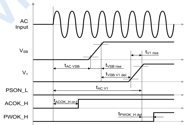
Figure 10. AC turn-on timing
