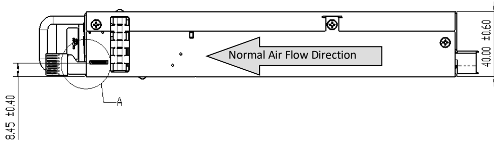
Figure 18. Side View
