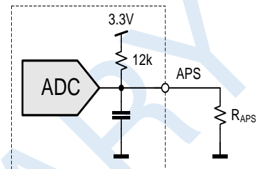
Figure 17. I2C address and protocol setting
