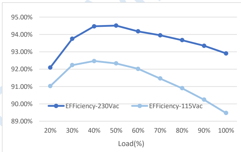
Figure 4. Efficiency vs. Load
