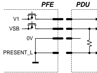
Figure 9. PRESENT_L signal pin
