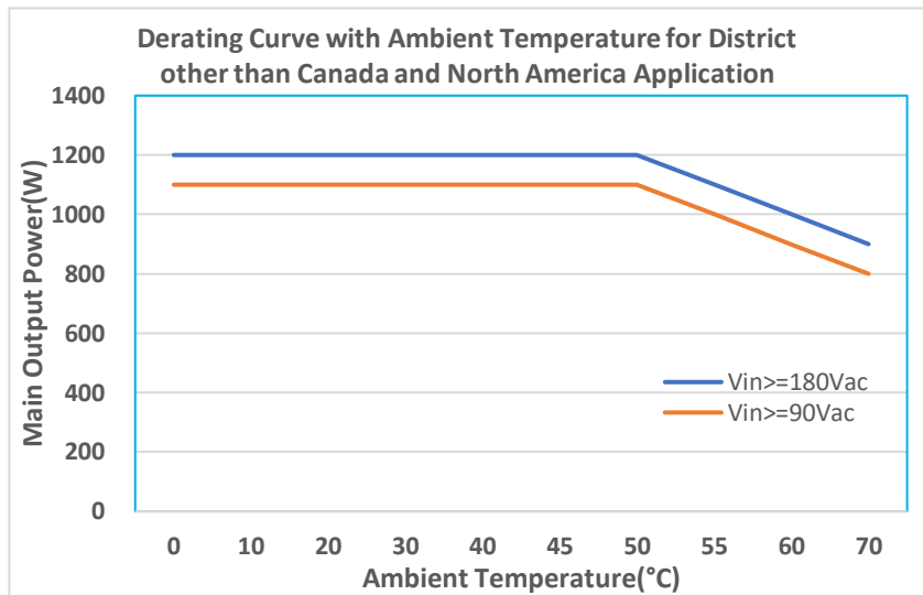
Figure 6b. I out Derating Curve for ambient above 50°C
