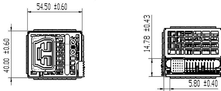
Figure 22. Front and Rear View
