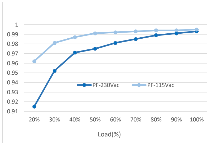
Figure 3. PF vs. Load
