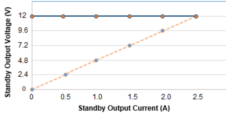
Figure 7. Current Limitation on 12 V SB
