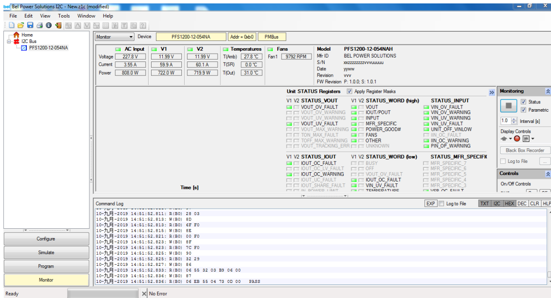
Figure 19. Monitoring dialog of the I2C Utility
