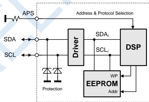
Figure 18. I2C Bus to DPS and EEPROM
