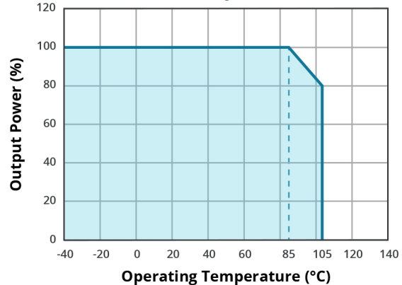
TEMPERATURE DERATING CURVE all other input models
