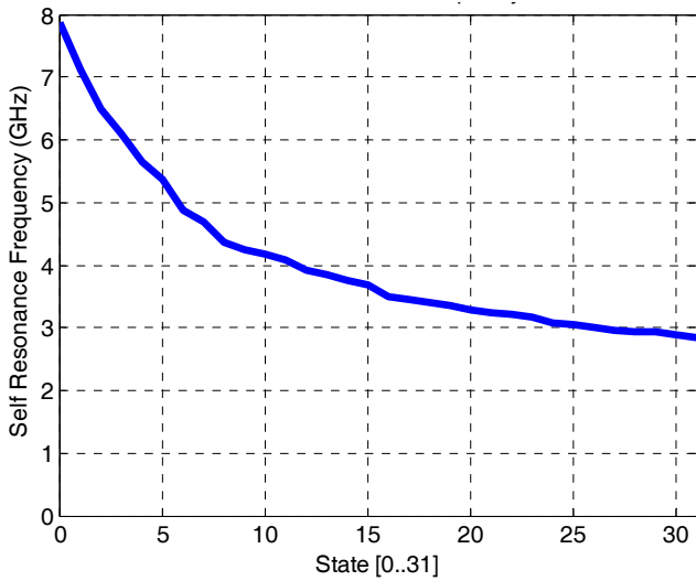
Figure 10. Measured Self Resonance Frequency
