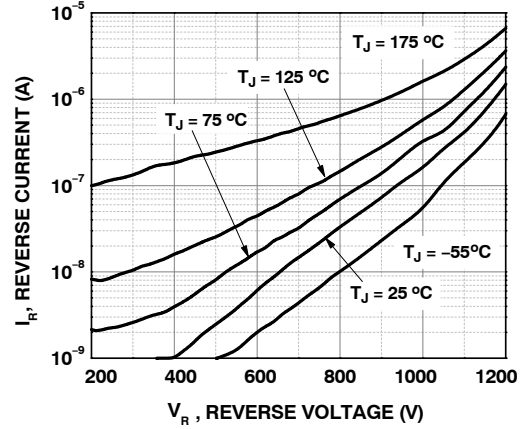
Figure 3. Reverse Characteristics
