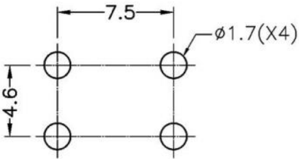
MOUNTING HOLES
