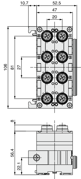
EX600-DX□D
