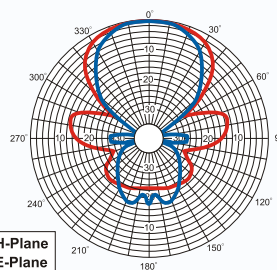
Typical 6 Element
