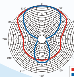
Typical 4 Element
