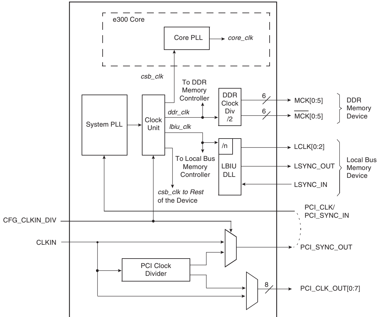
Figure 19-1. PC8349/E Clock Subsystem
