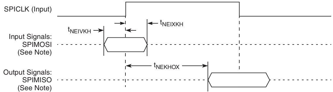
Figure 17-2. SPI AC Timing in Slave Mode (External Clock) Diagram
