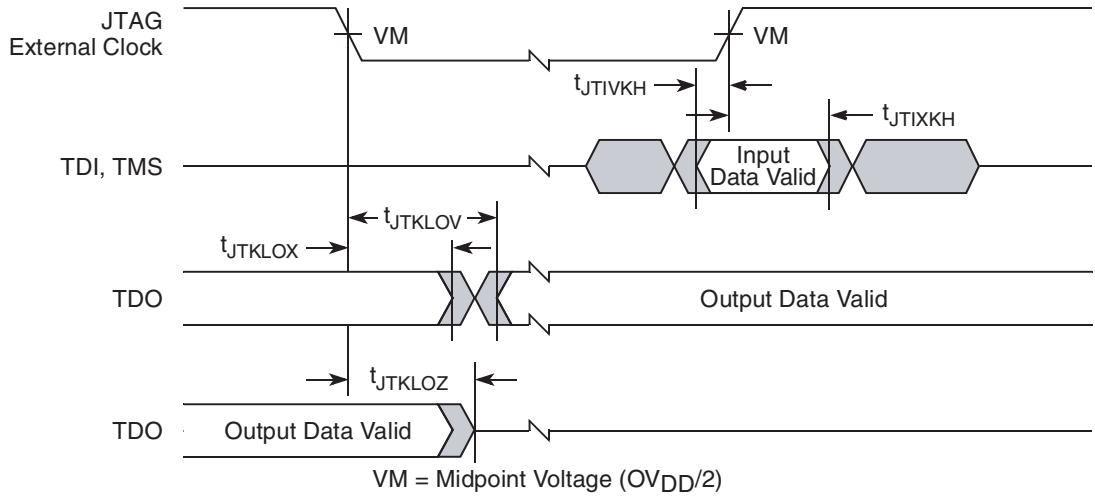
Figure 11-5. Test Access Port Timing Diagram
