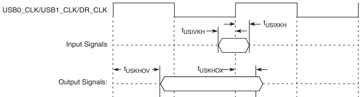
Figure 9-2. USB Signals
