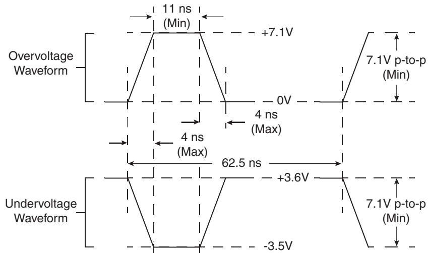
Figure 2-2. Maximum AC Waveforms on PCI Interface for 3.3-V Signaling
