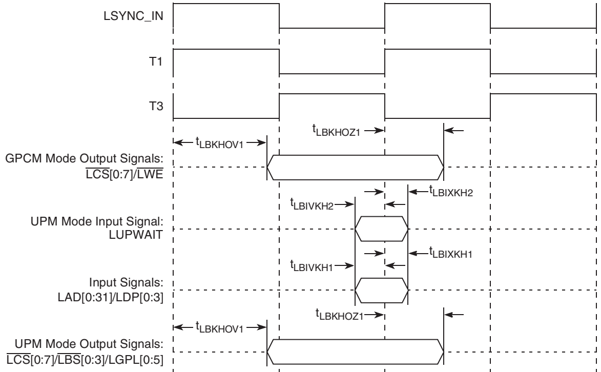
Figure 10-4. Local Bus Signals, GPCM/UPM Signals for LCCR[CLKDIV] = 2 (DLL Enabled)
