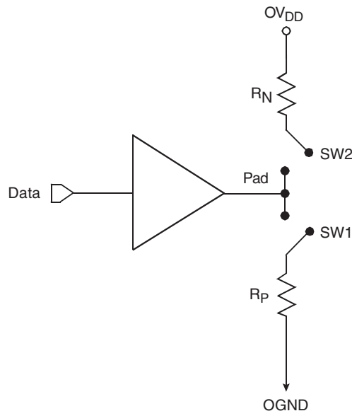
Figure 21-2. Driver Impedance Measurement
