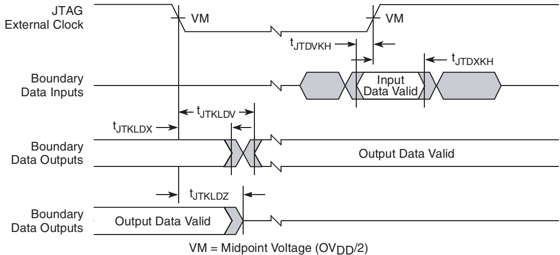
Figure 11-4. Boundary-Scan Timing Diagram
