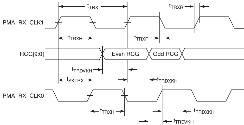
Figure 8-7. TBI Receive AC Timing Diagram
