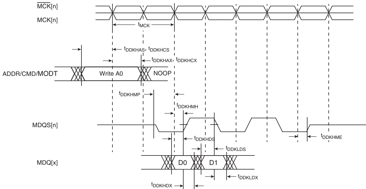
Figure 6-3. DDR SDRAM Output Timing Diagram
