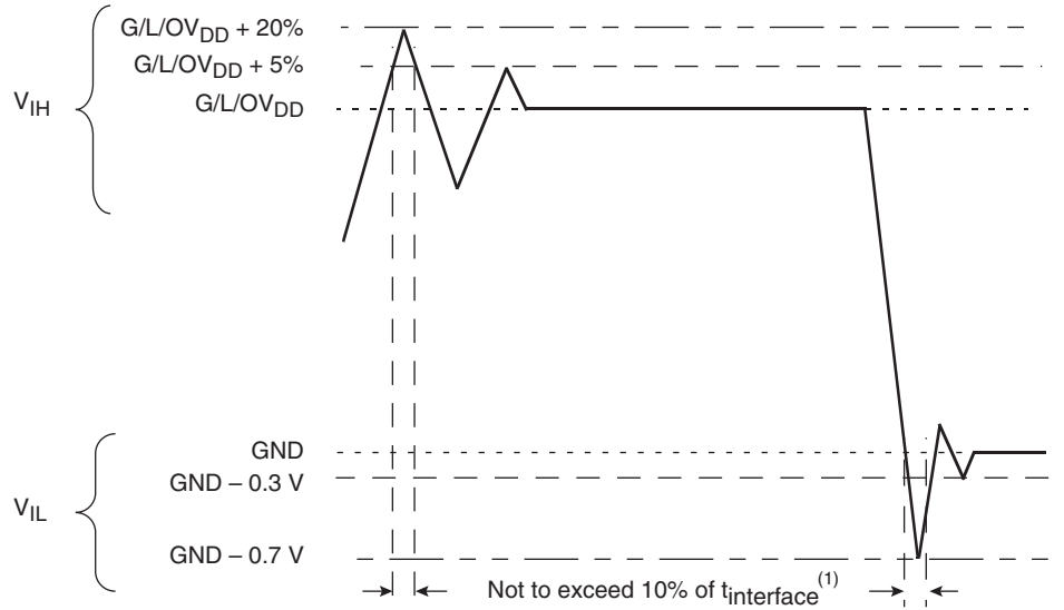
Figure 2-1. Overshoot/Undershoot Voltage for G_{V_{DD}}/O_{V_{DD}}/L_{V_{DD}}
