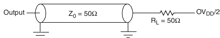
Figure 17-1. SPI AC Test Load
