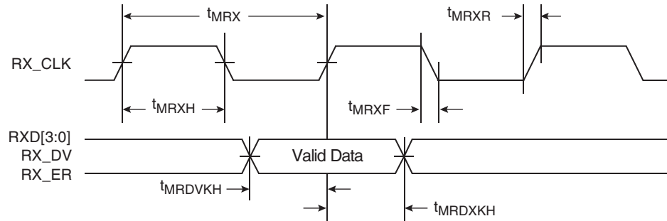
Figure 8-5. MII Receive AC Timing Diagram
