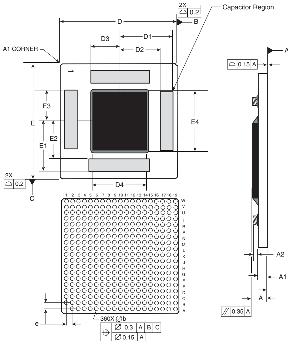
Figure 8-2. Mechanical Dimensions and Bottom Surface Nomenclature for the PC7448, 360 HiTCE LGA Package
