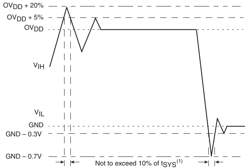
Figure 5-1. Overshoot/Undershoot Voltage
